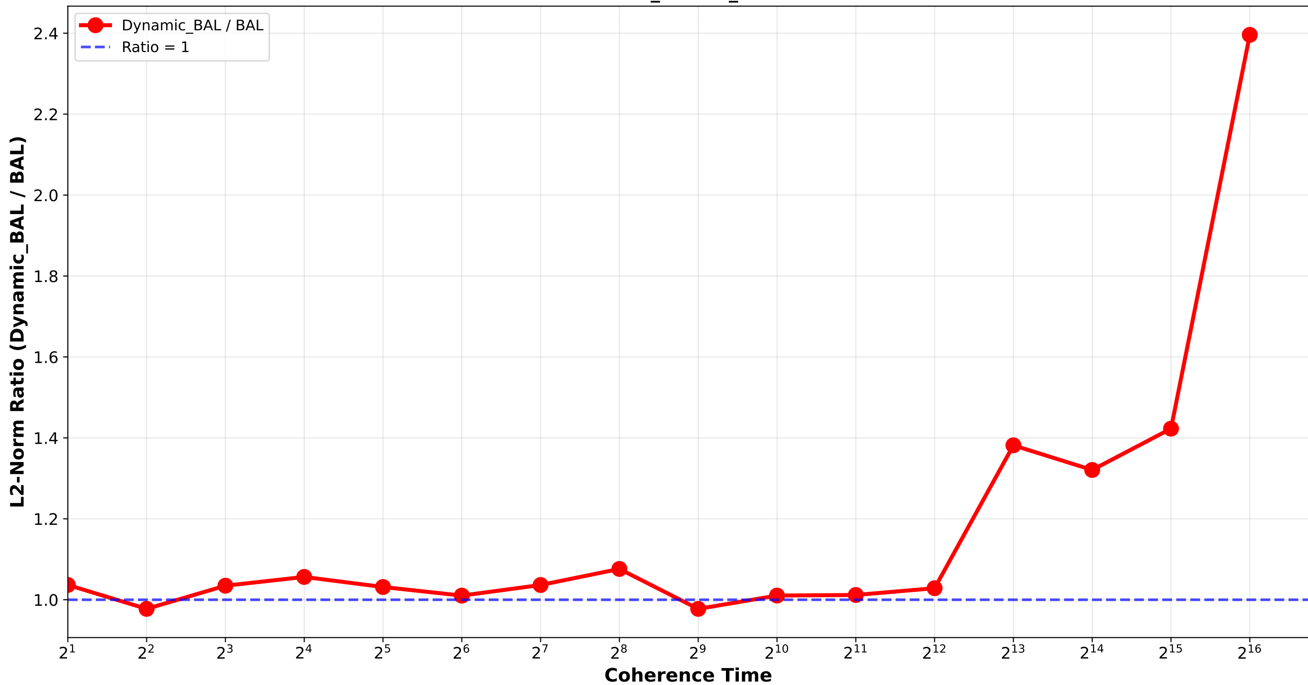
Dynamic_BAL vs BAL - L2 Norm Ratio Bounded_Pareto_random
