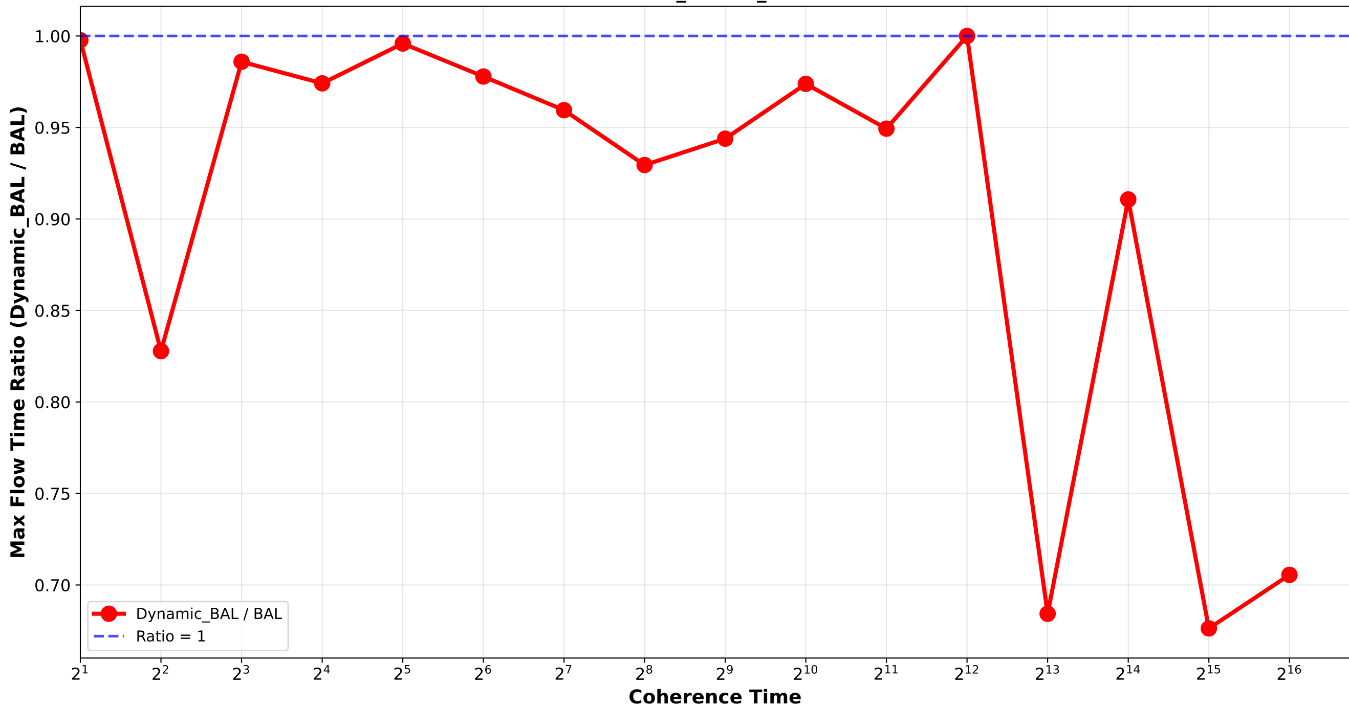
Dynamic_BAL vs BAL - Max Flow Time Ratio Bounded_Pareto_random
