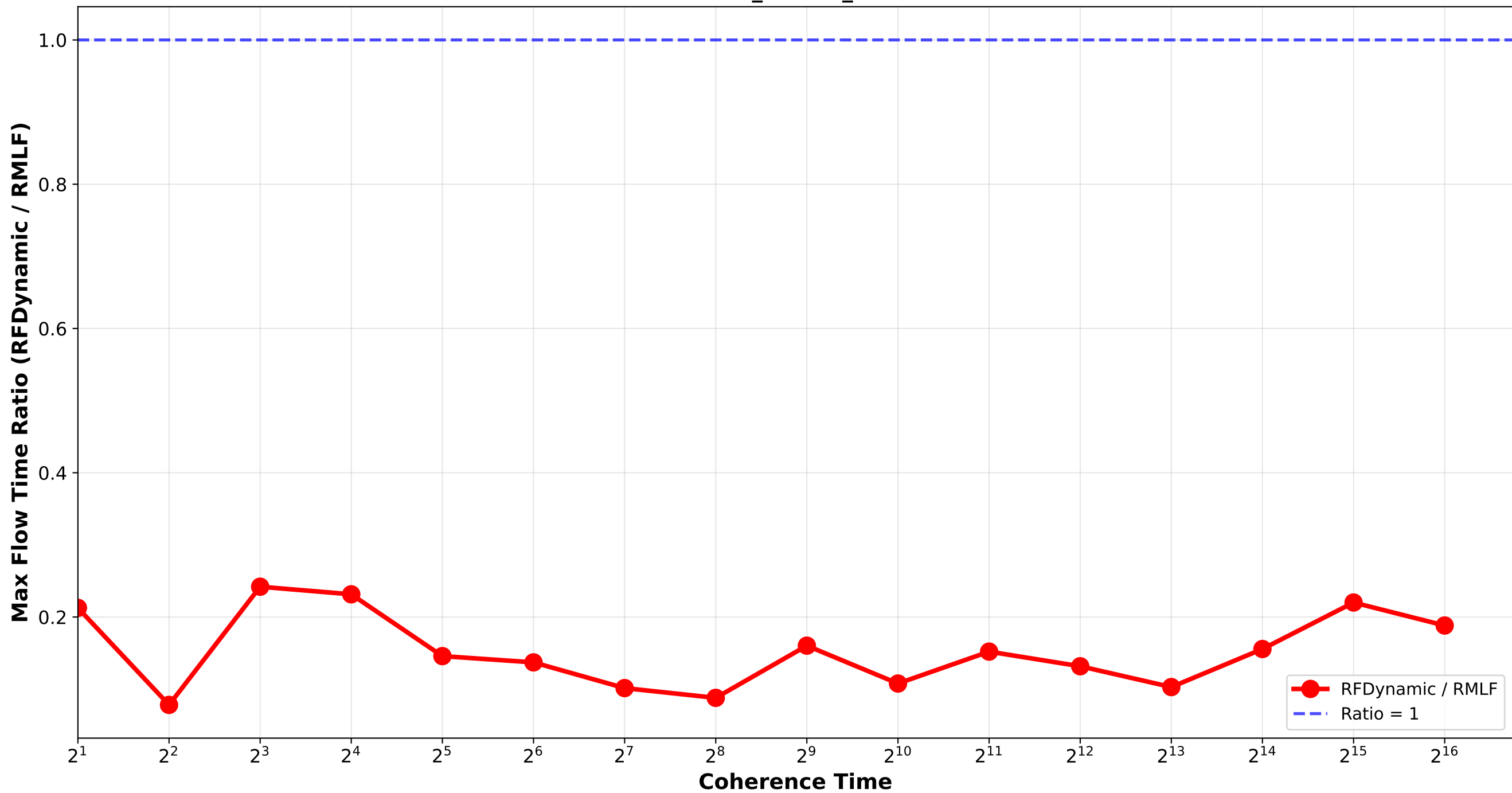
RFDynamic vs RMLF - Max Flow Time Ratio Bounded_Pareto_random
