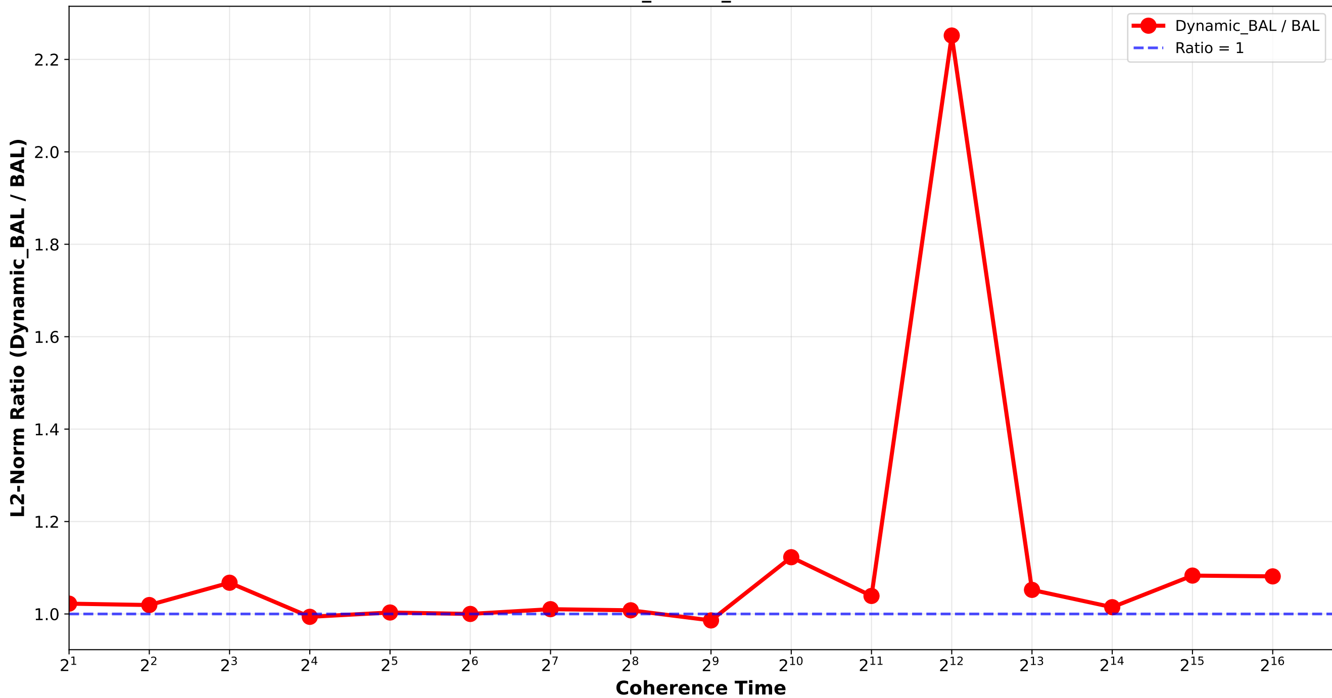
Dynamic_BAL vs BAL - L2 Norm Ratio Bounded_Pareto_softrandom
