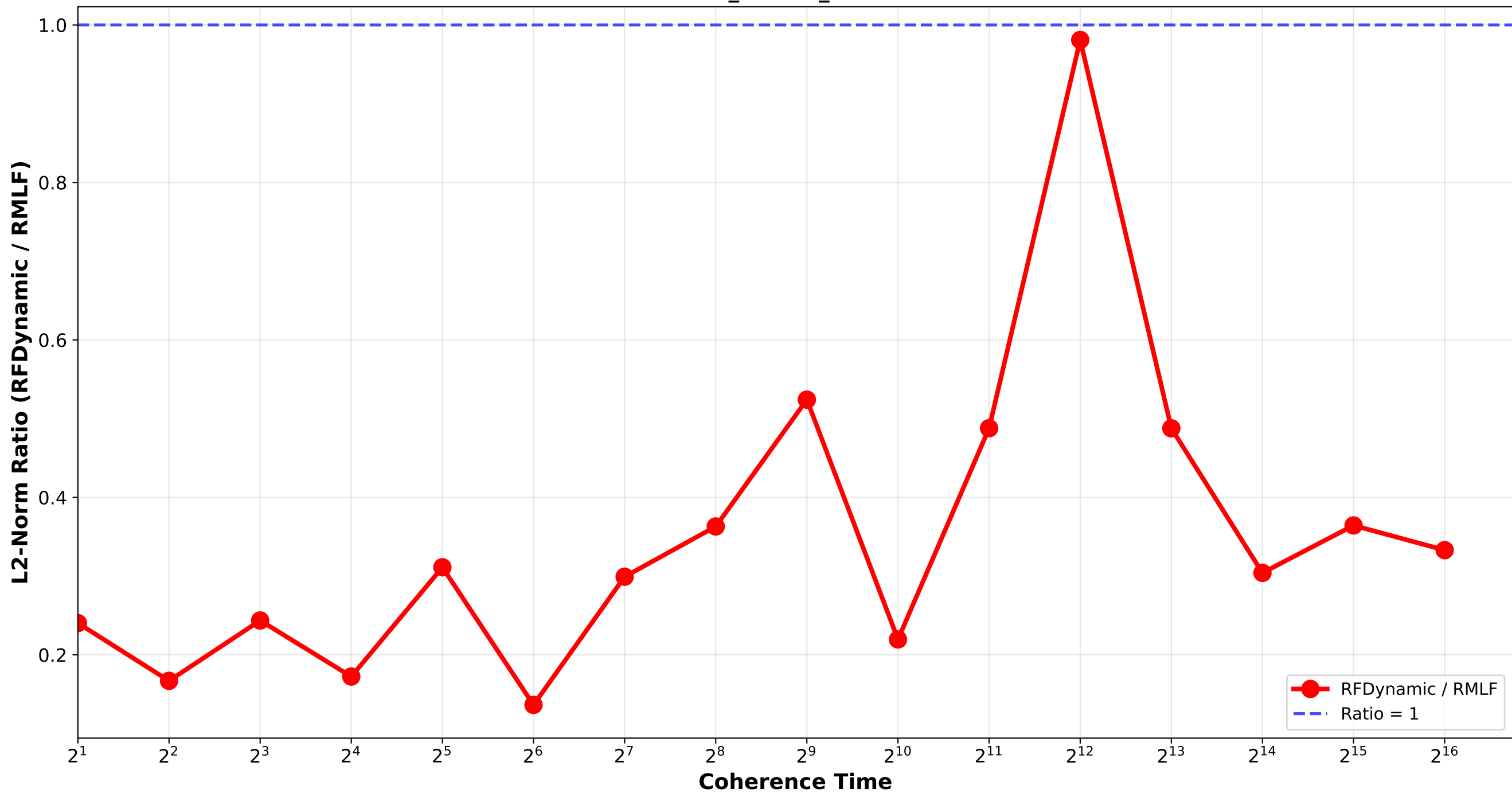
RFDynamic vs RMLF - L2 Norm Ratio Bounded_Pareto_softrandom
