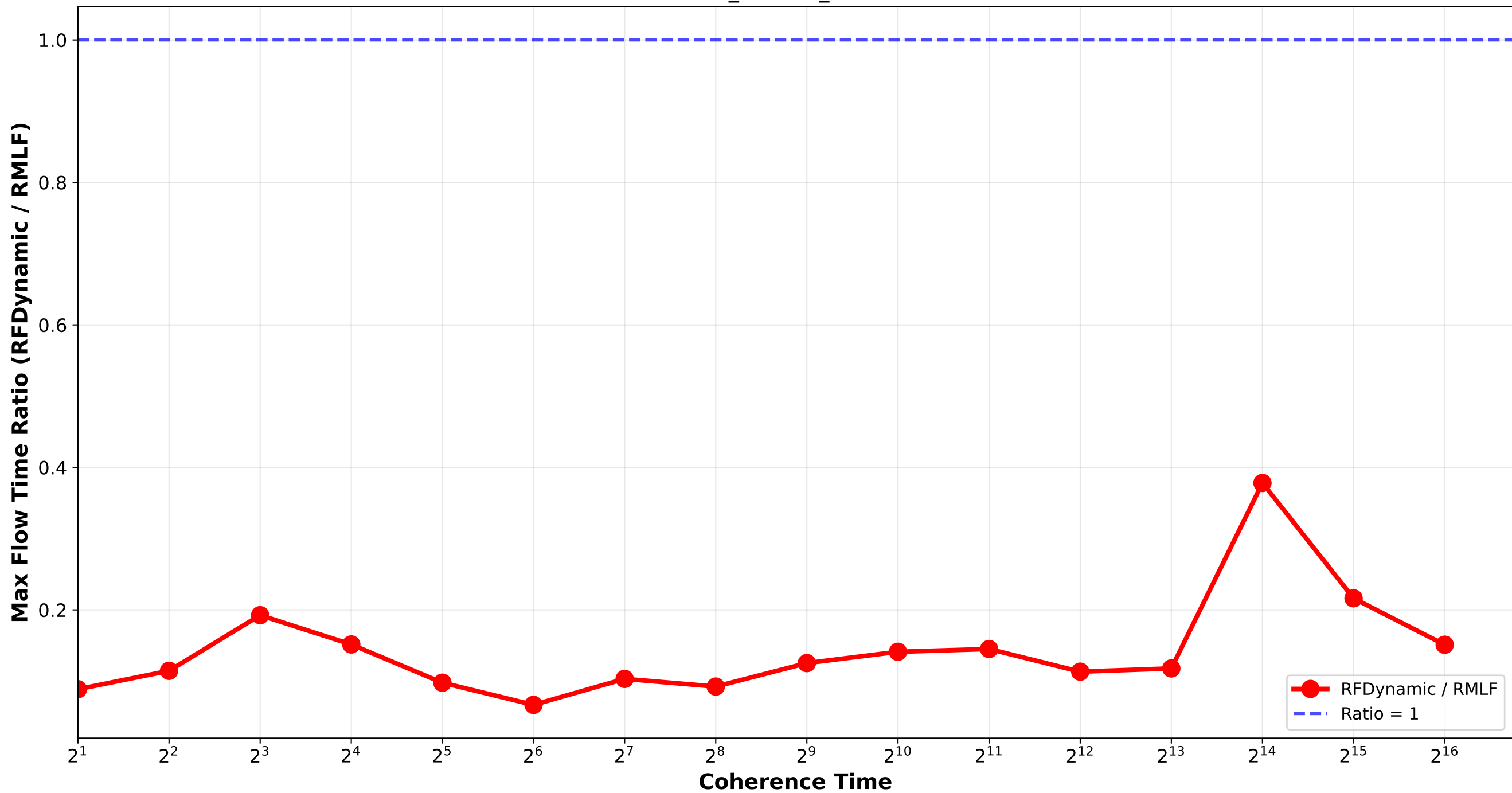
RFDynamic vs RMLF - Max Flow Time Ratio Bounded_Pareto_softrandom
