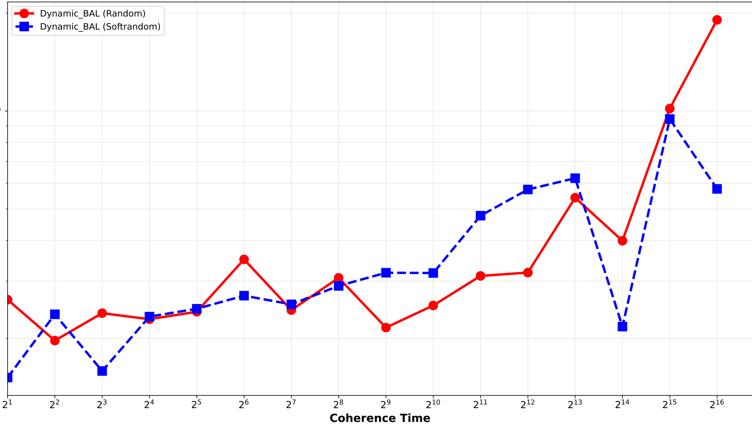
Dynamic_BAL: Random vs Softrandom
