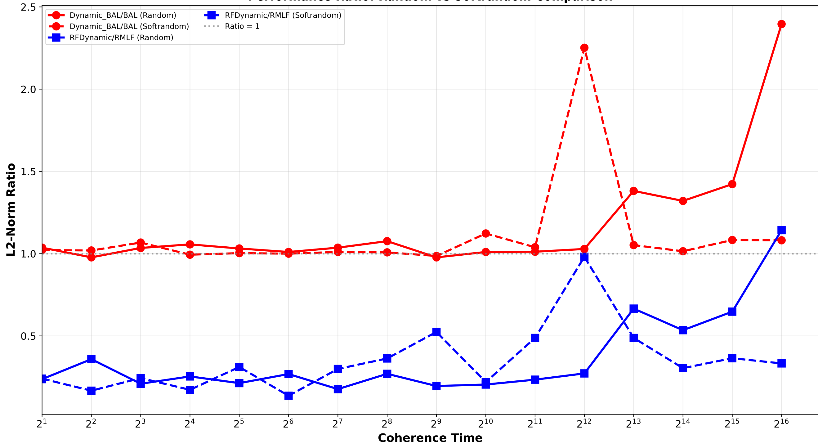
Performance Ratio: Random vs Softrandom Comparison
