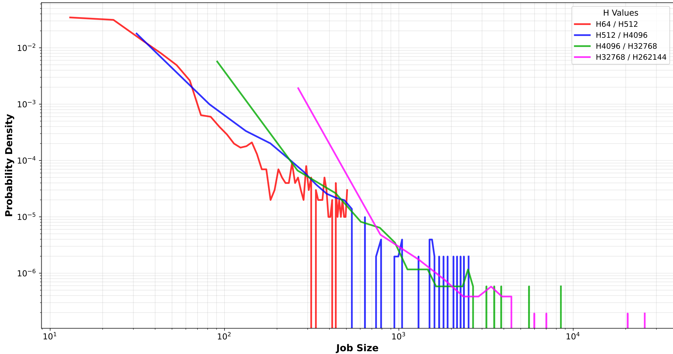
Job Size Distribution (Bounded Pareto) Different H Value Combinations
