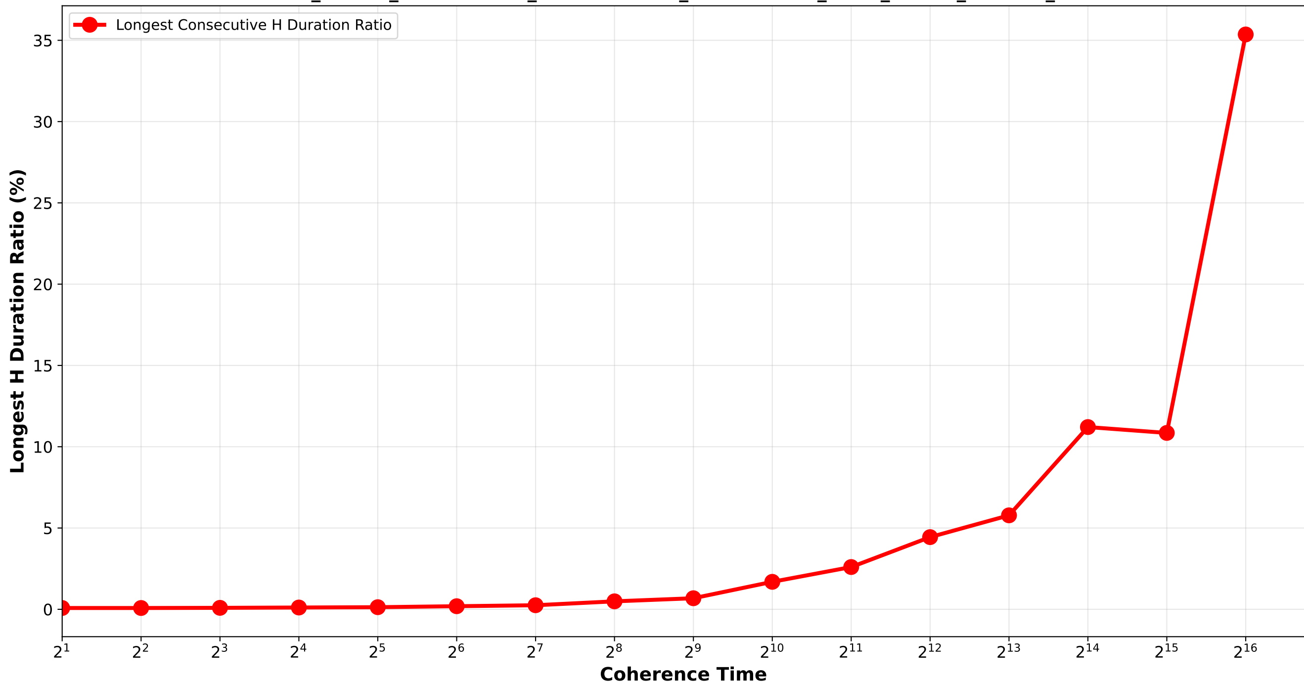
Longest Consecutive H Duration Ratio Bounded_Pareto_combination_random / four_combination_H512_H4096_H32768_H262144
