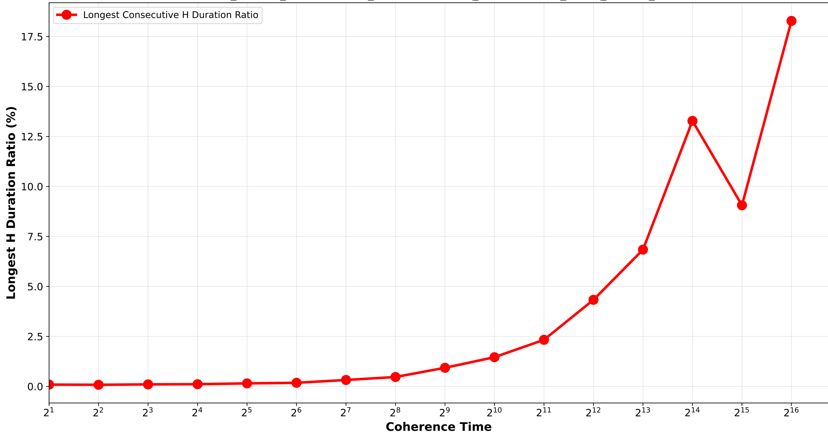
Longest Consecutive H Duration Ratio Bounded_Pareto_combination_random / three_combination_H512_H4096_H32768
