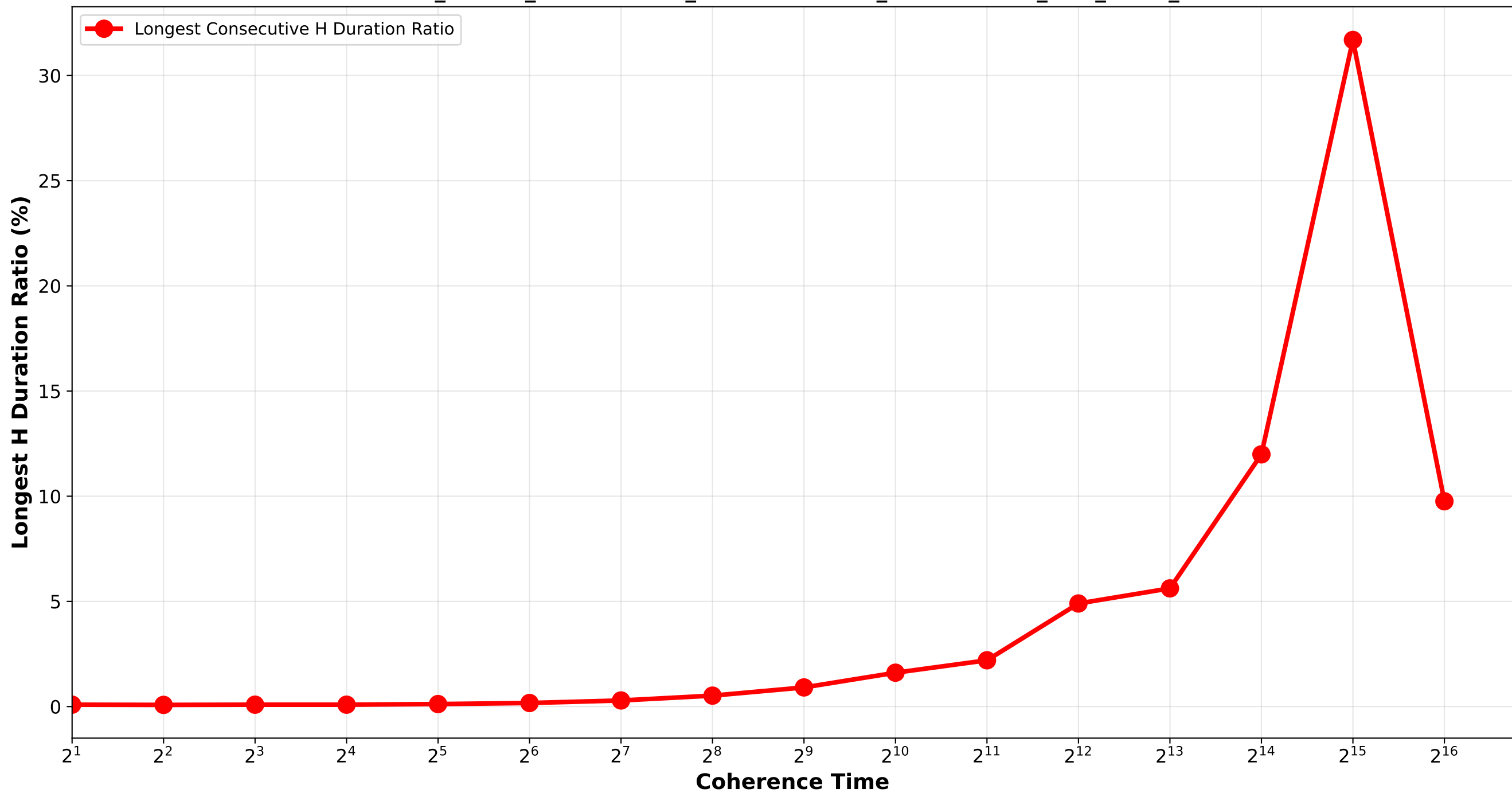
Longest Consecutive H Duration Ratio Bounded_Pareto_combination_random / three_combination_H64_H512_H4096
