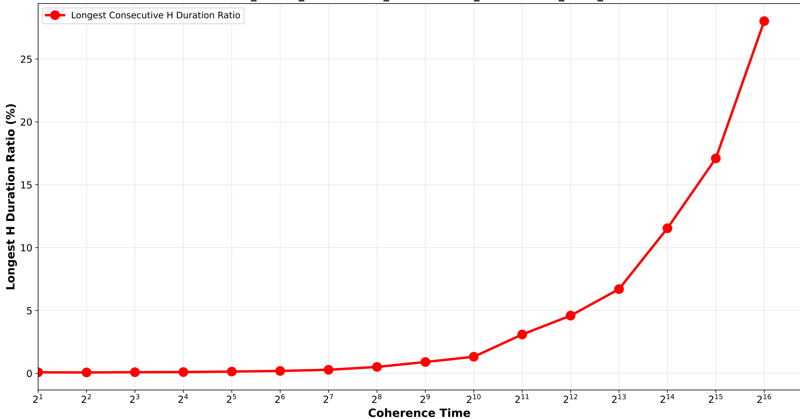
Longest Consecutive H Duration Ratio Bounded_Pareto_combination_random / two_combination_H512_H4096
