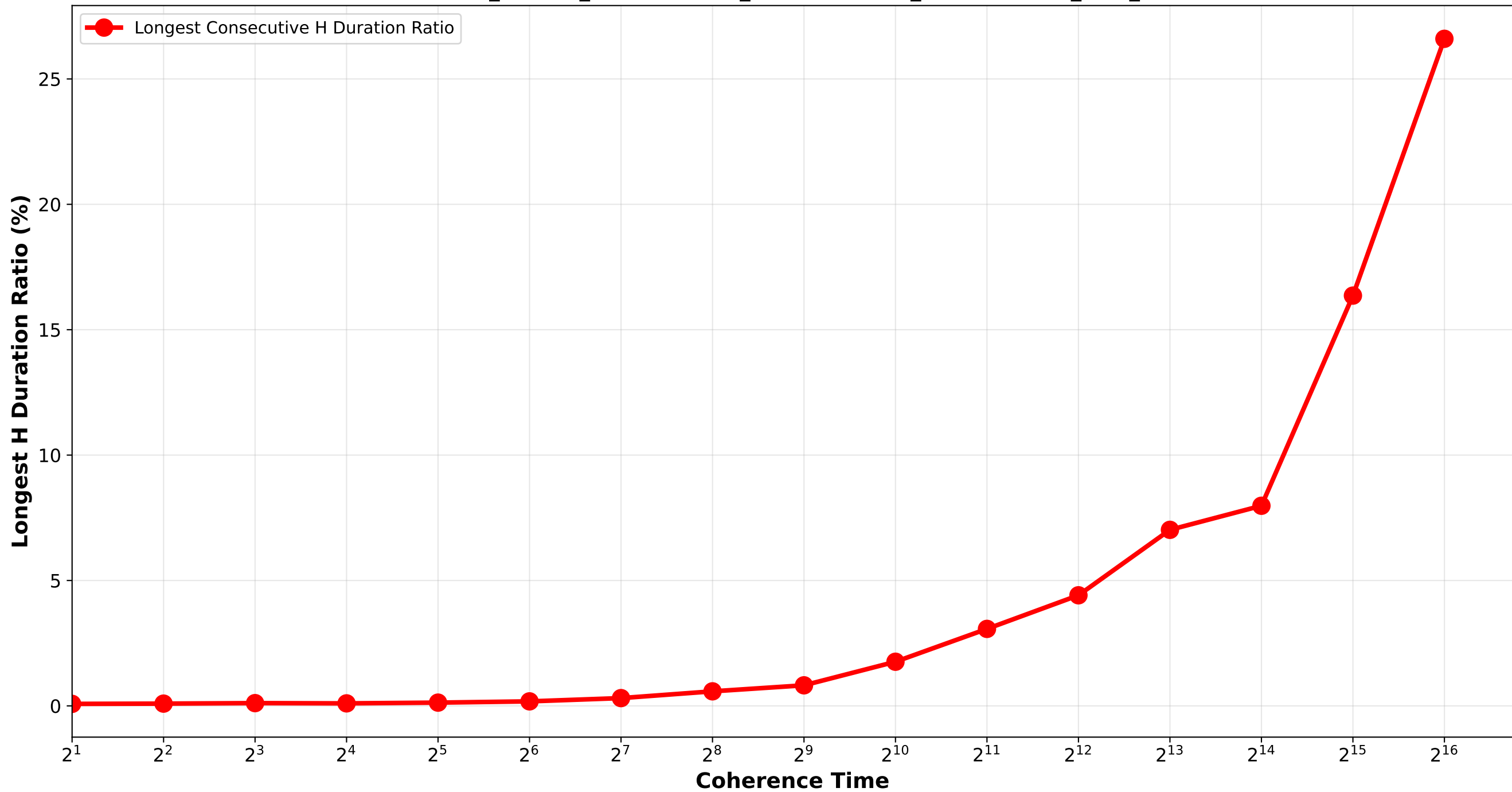
Longest Consecutive H Duration Ratio Bounded_Pareto_combination_random / two_combination_H64_H512
