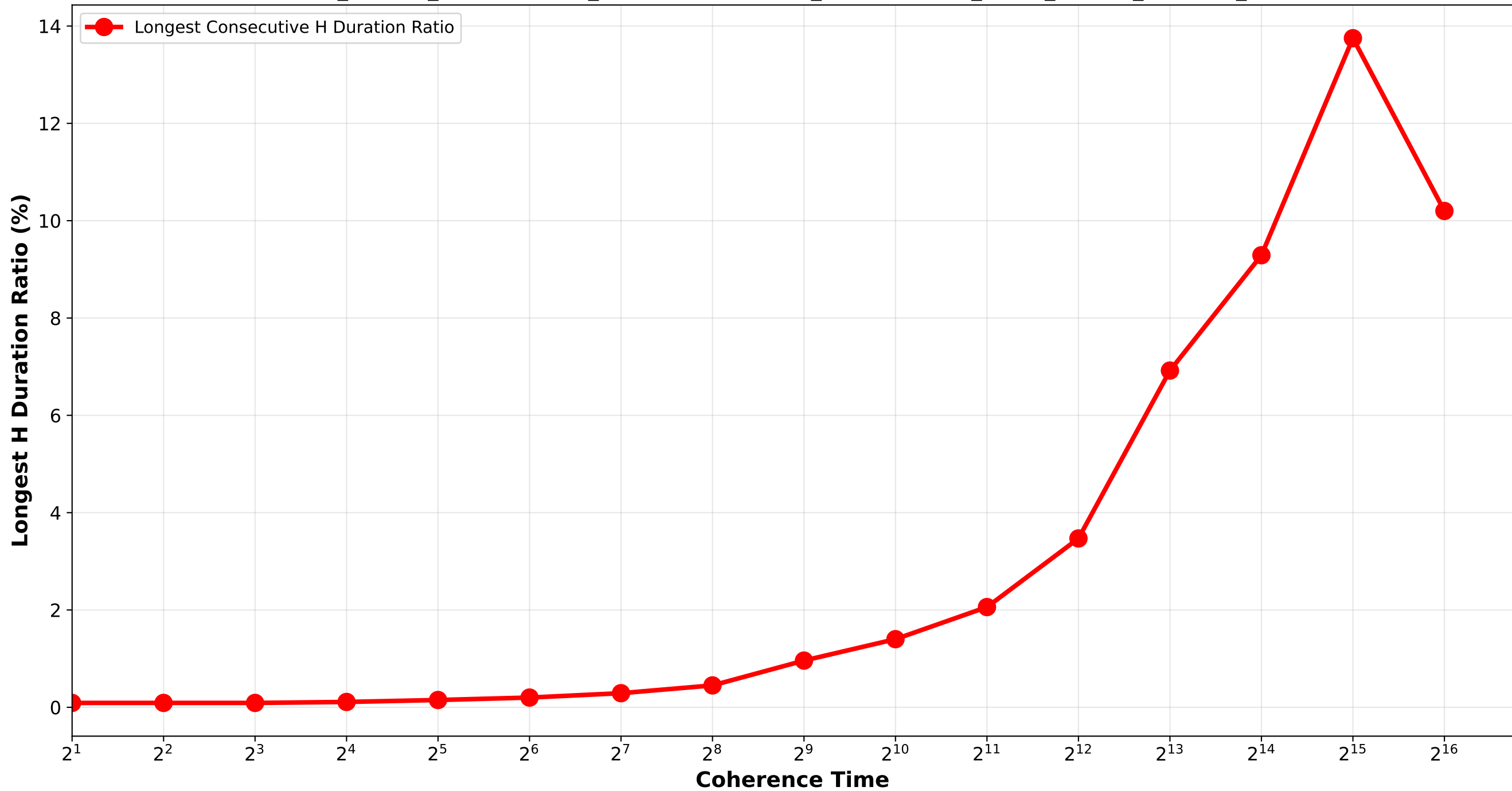
Longest Consecutive H Duration Ratio Bounded_Pareto_combination_softrandom / four_combination_H512_H4096_H32768_H262144
