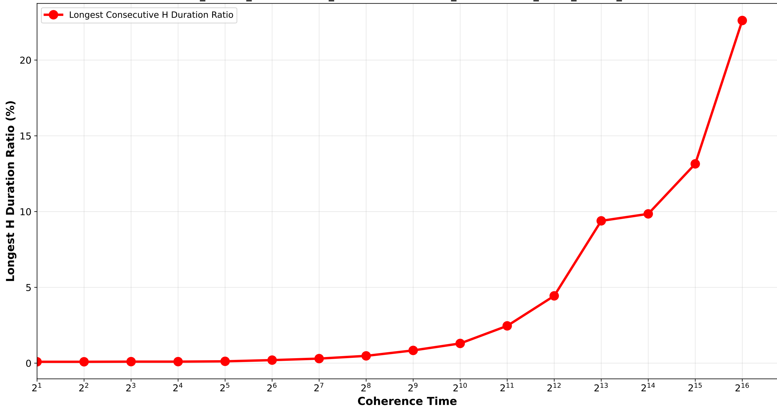
Longest Consecutive H Duration Ratio Bounded_Pareto_combination_softrandom / three_combination_H512_H4096_H32768
