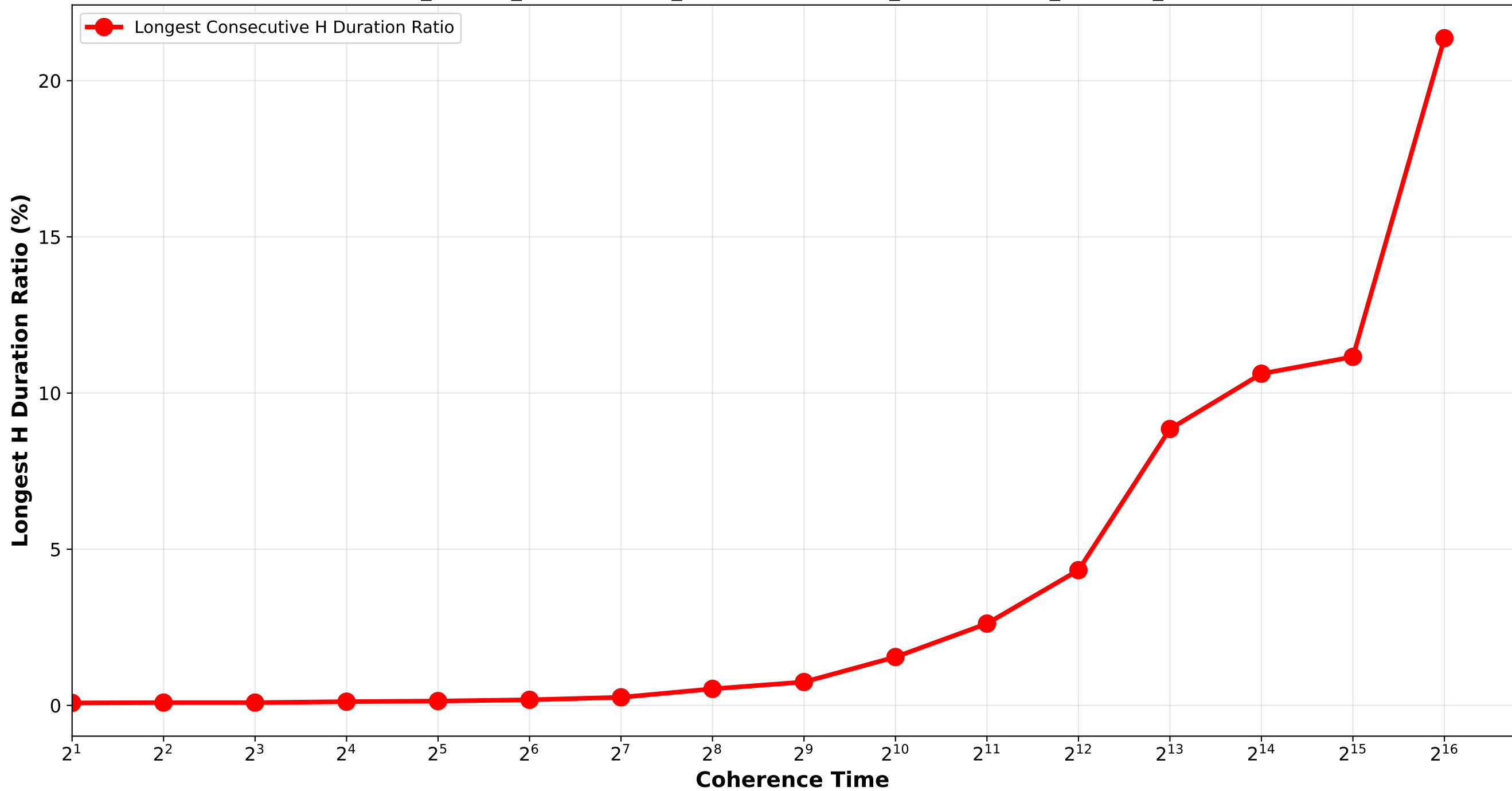
Longest Consecutive H Duration Ratio Bounded_Pareto_combination_softrandom / two_combination_H32768_H262144
