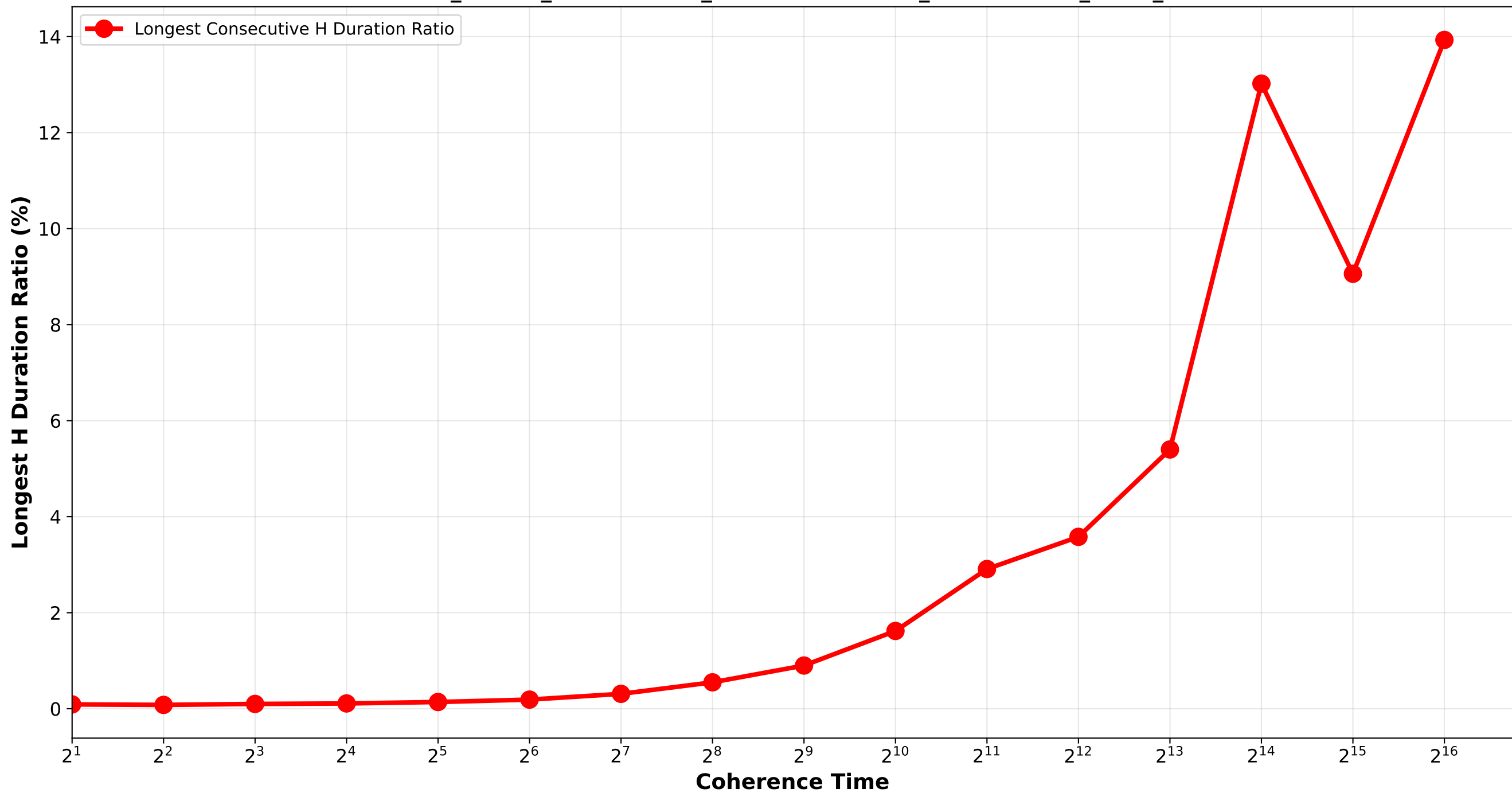
Longest Consecutive H Duration Ratio Bounded_Pareto_combination_softrandom / two_combination_H512_H4096
