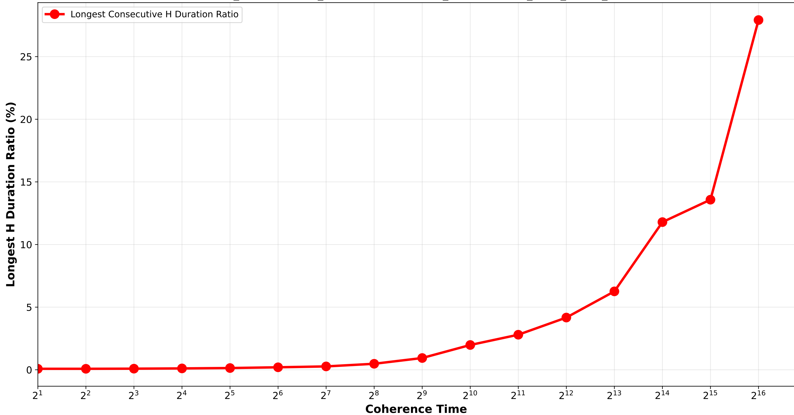
Longest Consecutive H Duration Ratio normal_combination_softrandom / three_combination_std9_std12_std15
