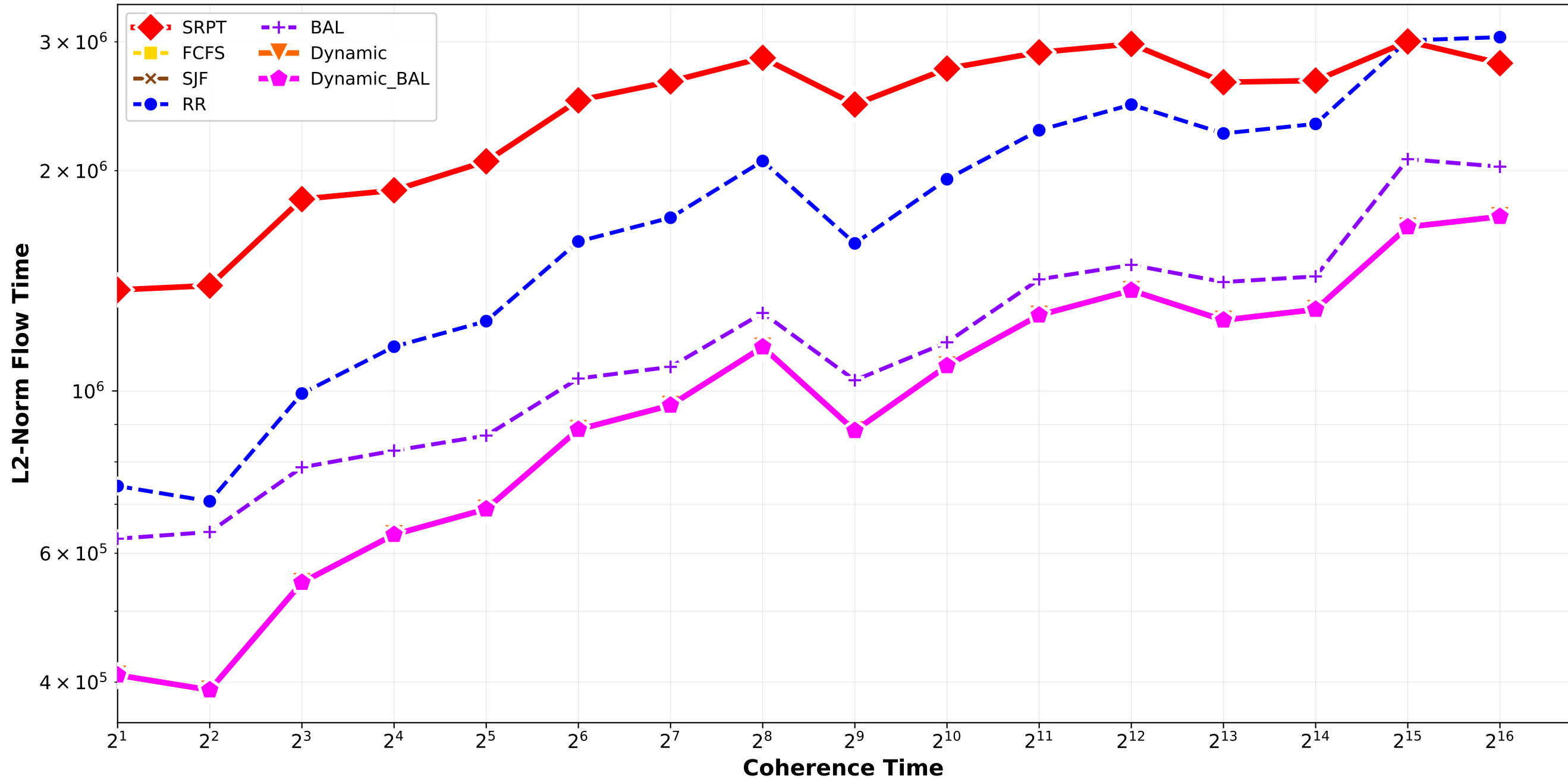
Clairvoyant Algorithms - L2 Norm Flow Time normal_combination_random std6_std9_std12_std15 / quadruplet_1
