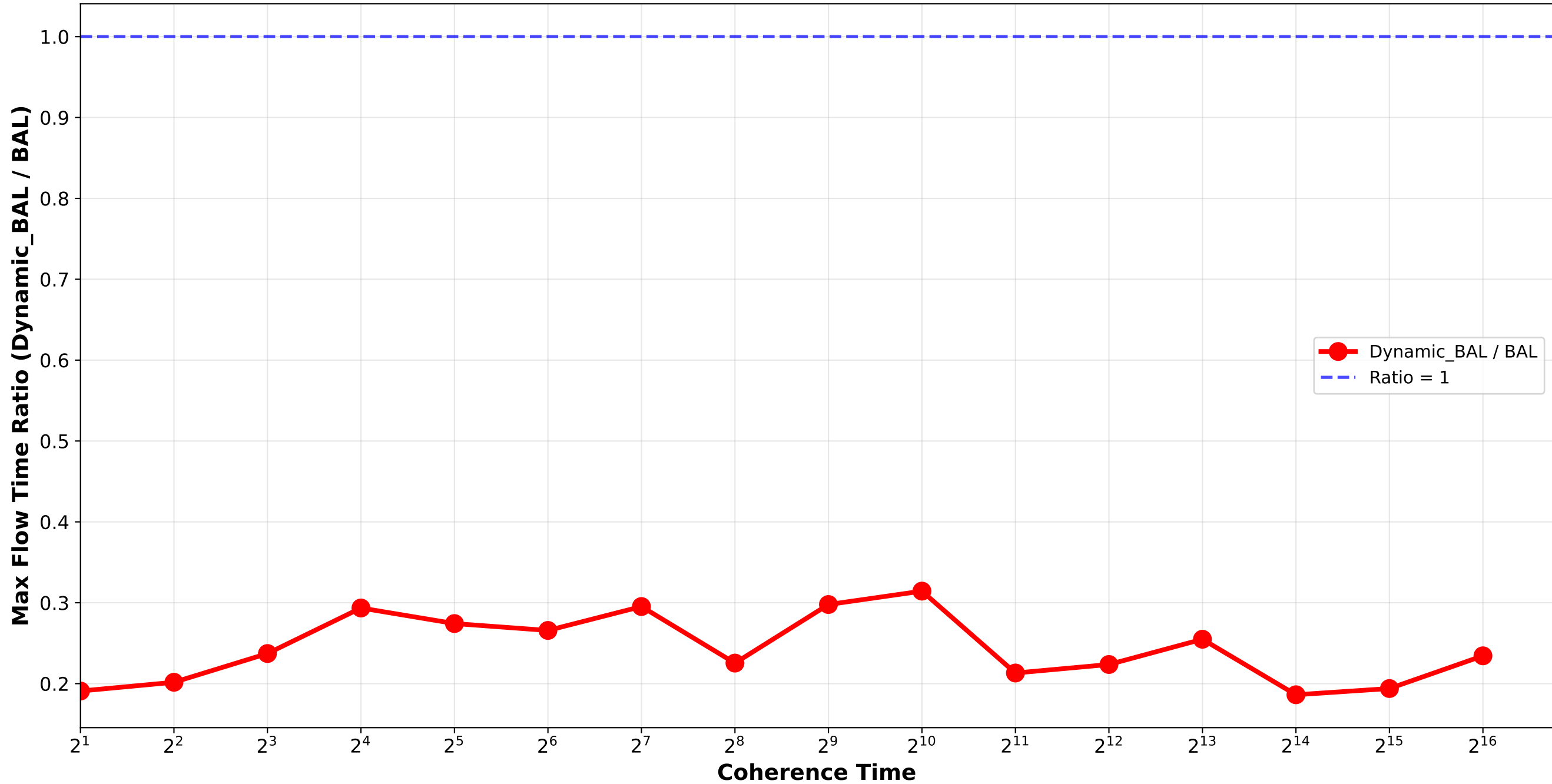
Dynamic_BAL vs BAL - Max Flow Time Ratio normal_combination_random std6_std9_std12_std15 / quadruplet_1
