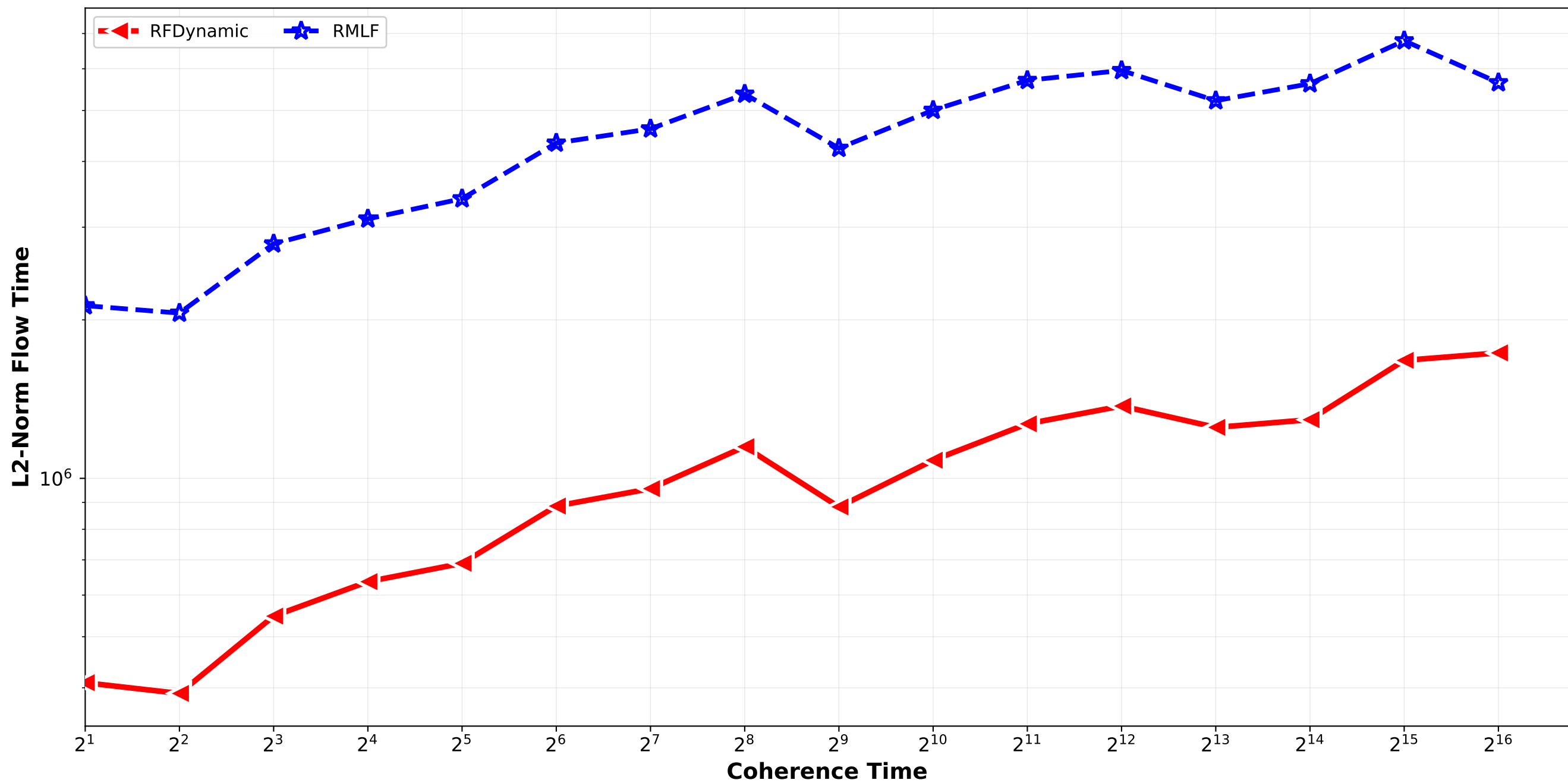
RFDynamic vs RMLF- L2 Norm Flow Time normal_combination_random std6_std9_std12_std15 / quadruplet_1
