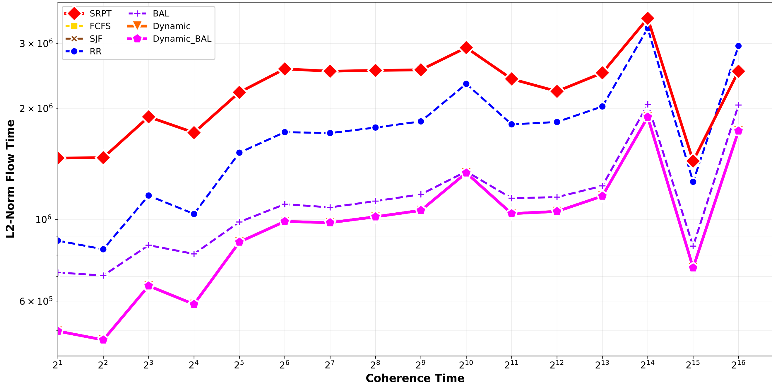
Clairvoyant Algorithms - L2 Norm Flow Time normal_combination_random std9_std12_std15_std18 / quadruplet_2
