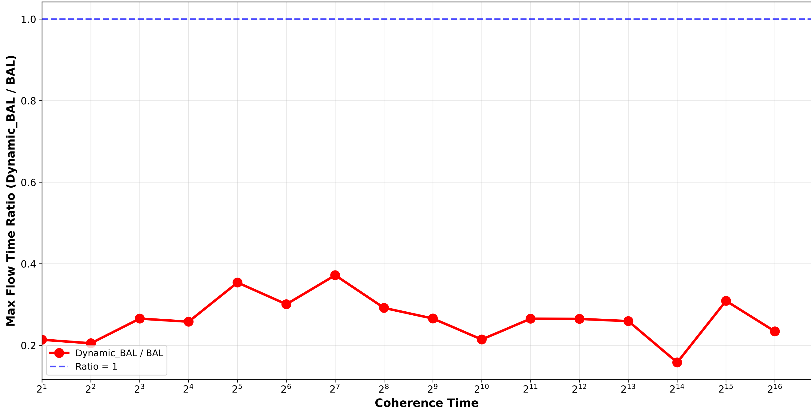
Dynamic_BAL vs BAL - Max Flow Time Ratio normal_combination_random std9_std12_std15_std18 / quadruplet_2
