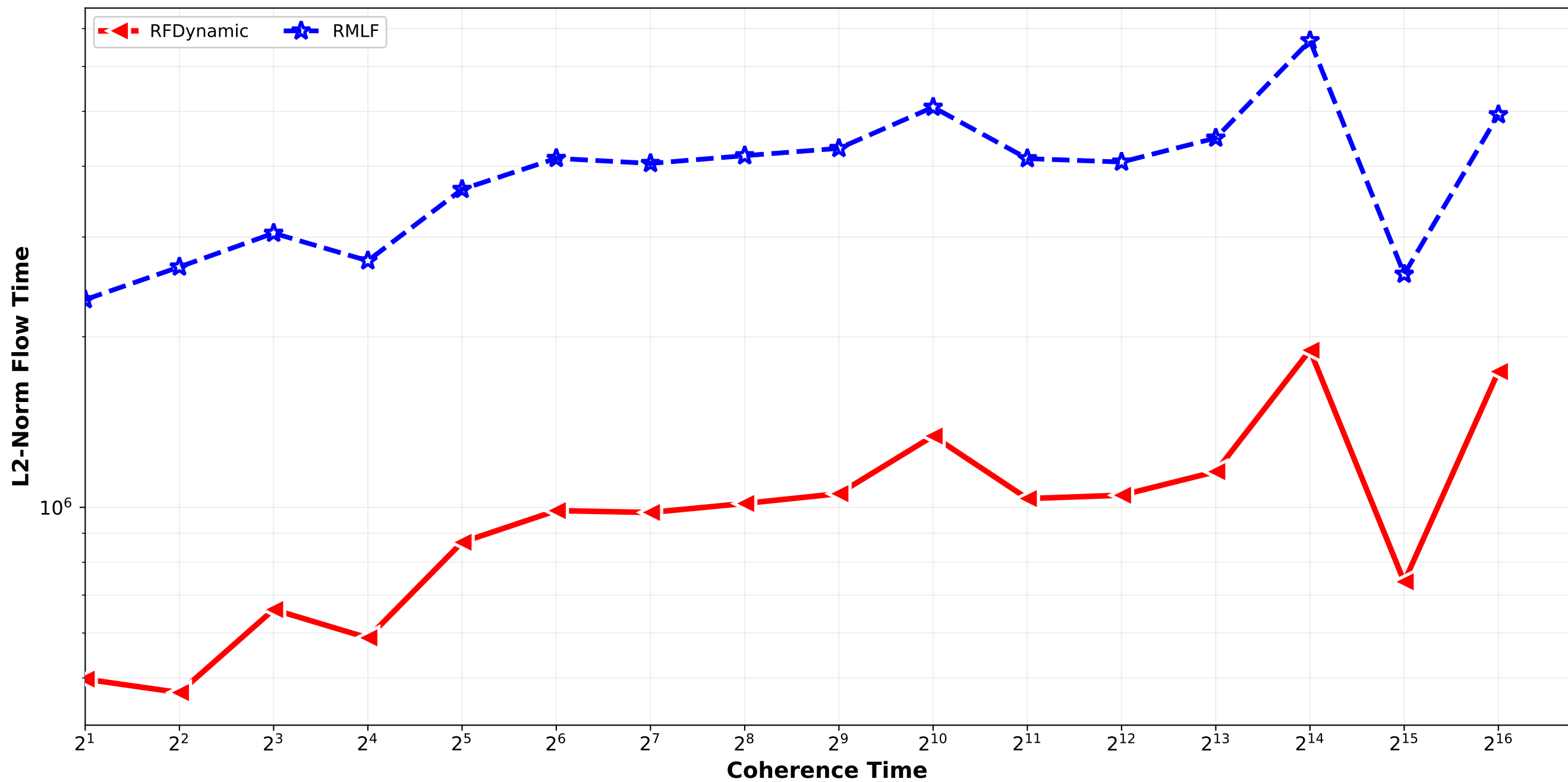
RFDynamic vs RMLF- L2 Norm Flow Time normal_combination_random std9_std12_std15_std18 / quadruplet_2
