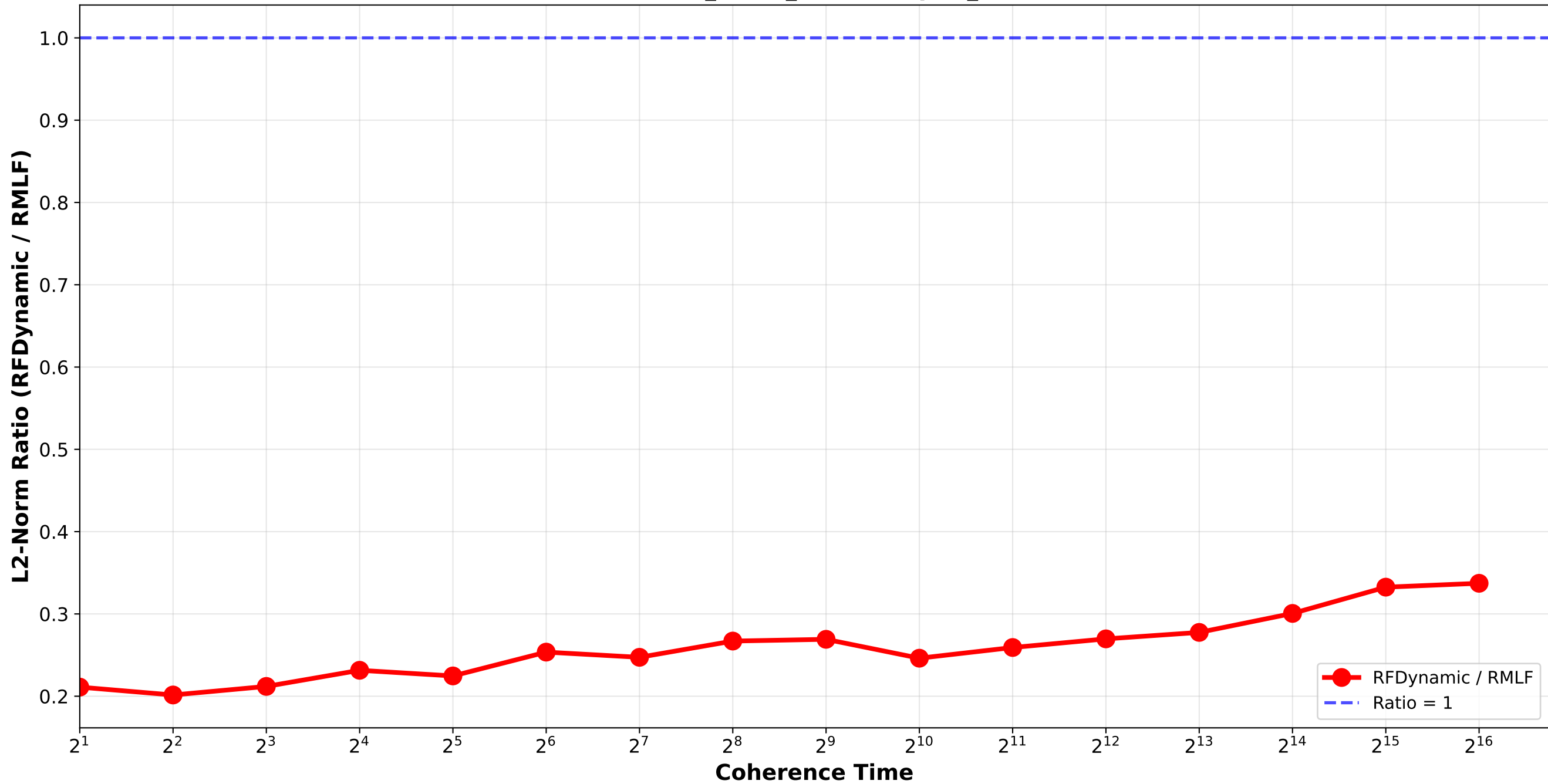
RFDynamic vs RMLF - L2 Norm Ratio normal_combination_random std12_std15_std18 / triplet_3
