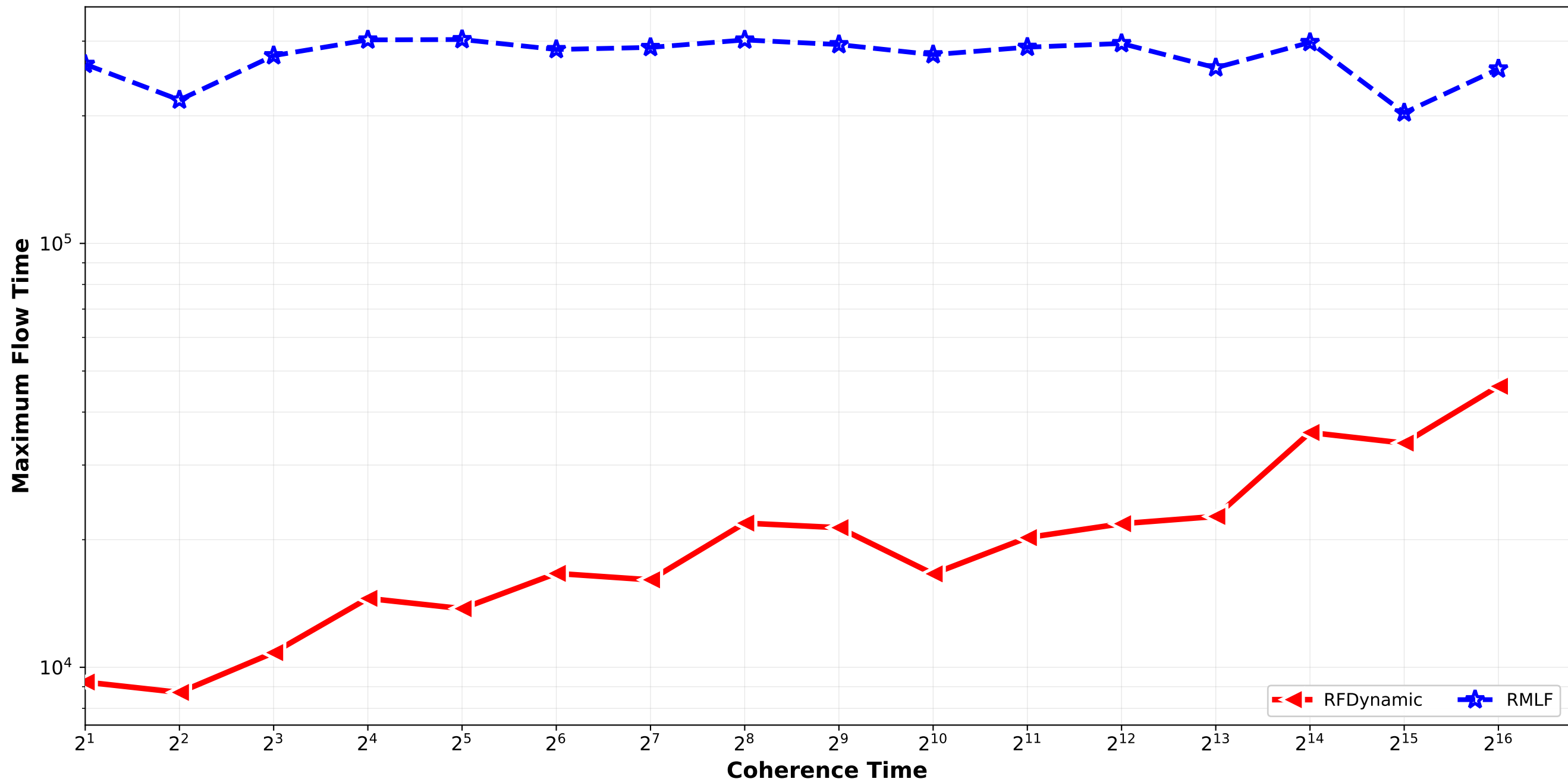
RFDynamic vs RMLF - Maximum Flow Time normal_combination_random std12_std15_std18 / triplet_3
