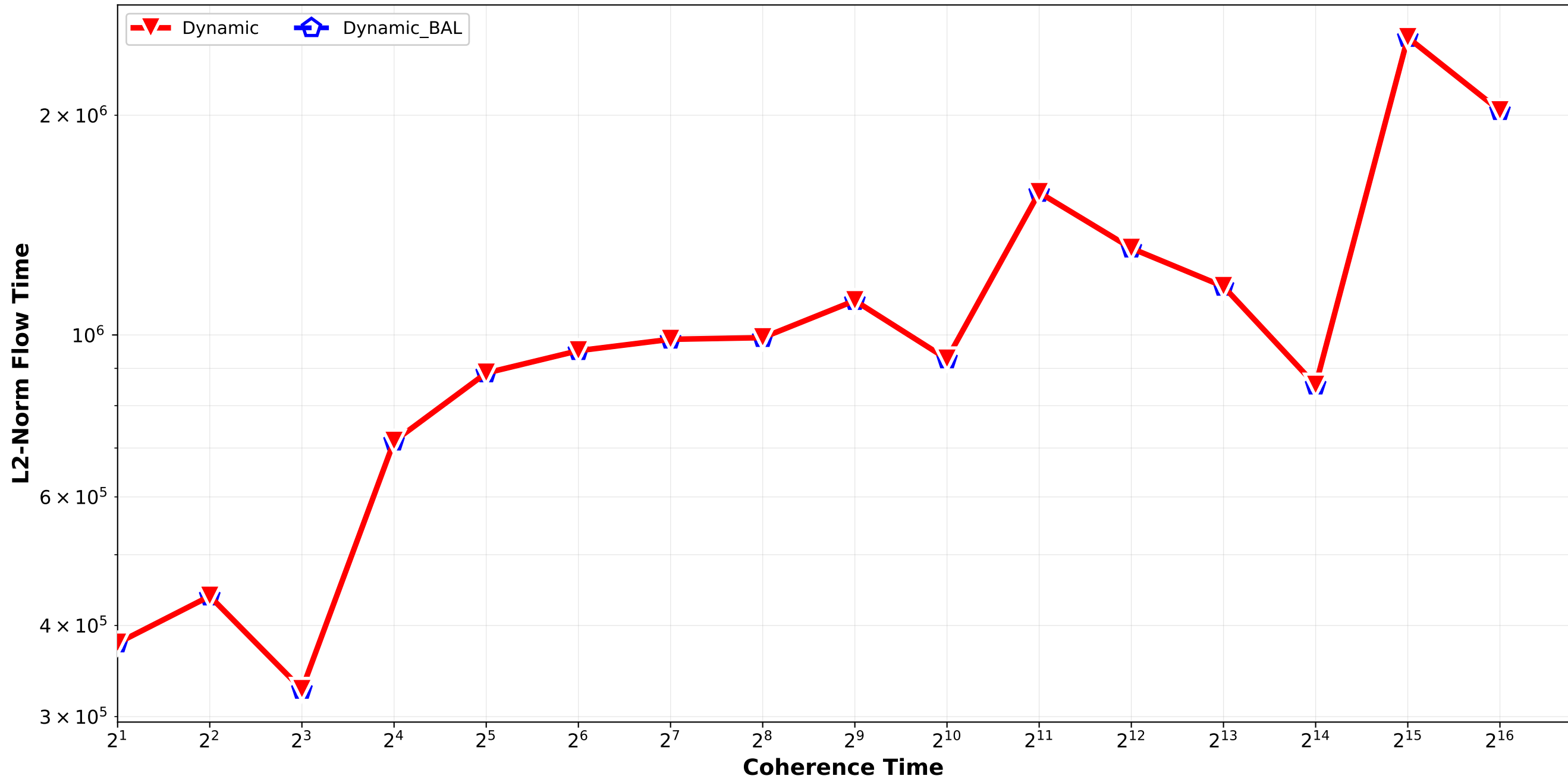
Dynamic vs Dynamic_BAL - L2 Norm Flow Time normal_combination_random std6_std9_std12 / triplet_1
