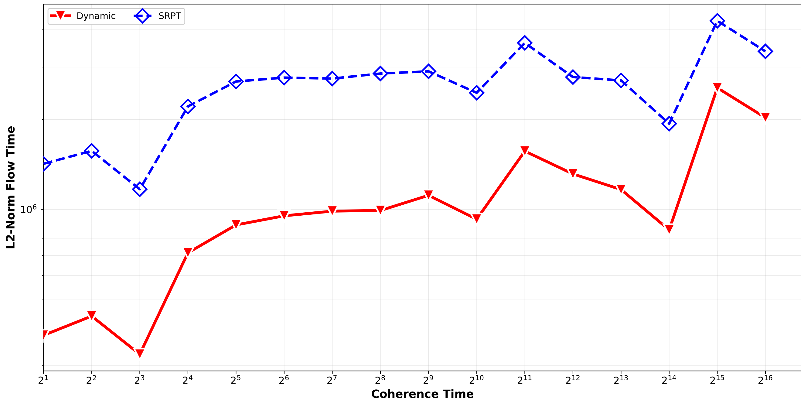
Dynamic vs SRPT - L2 Norm Flow Time normal_combination_random std6_std9_std12 / triplet_1
