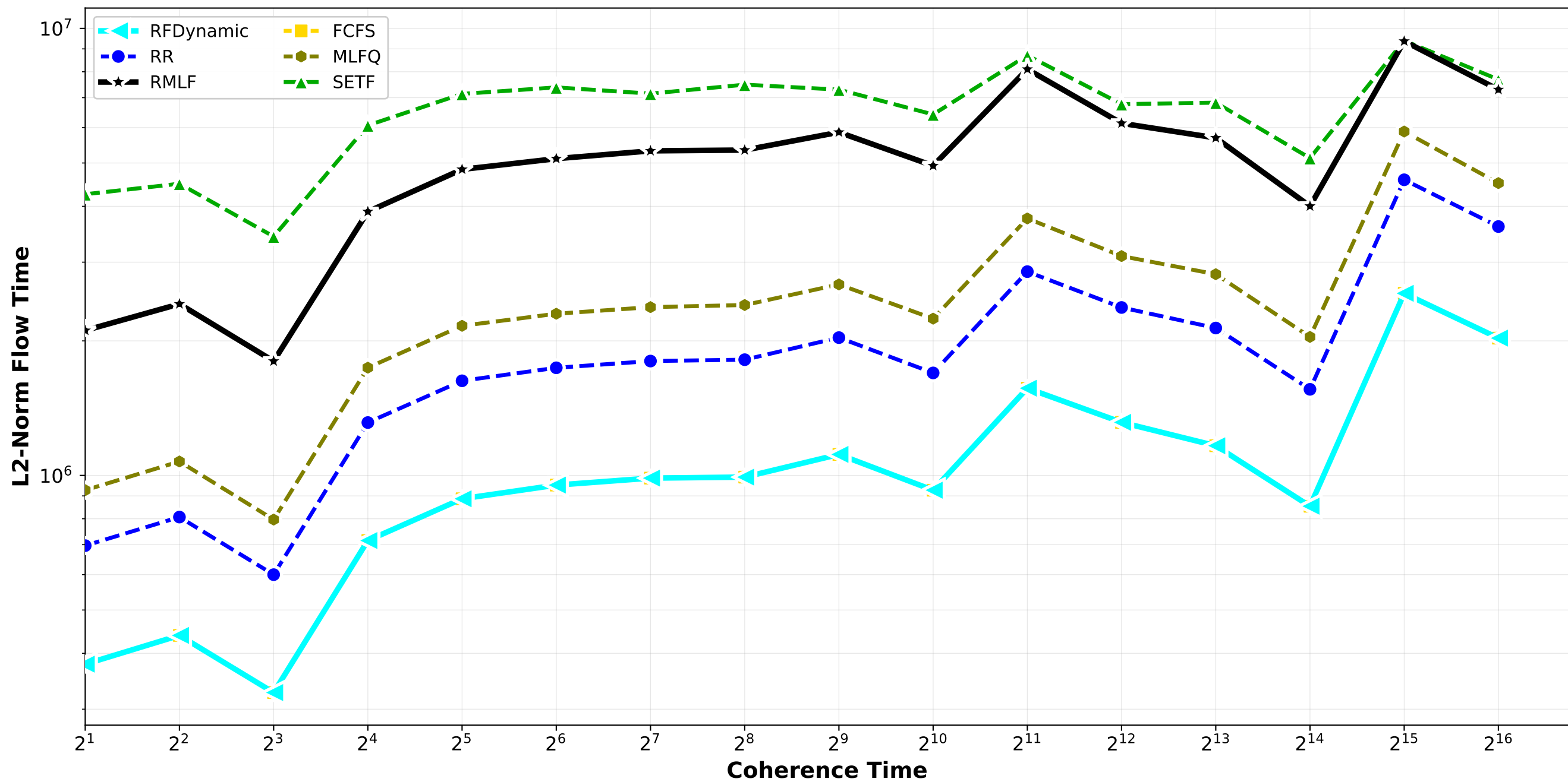
Non-Clairvoyant Algorithms - L2 Norm Flow Time normal_combination_random std6_std9_std12 / triplet_1
