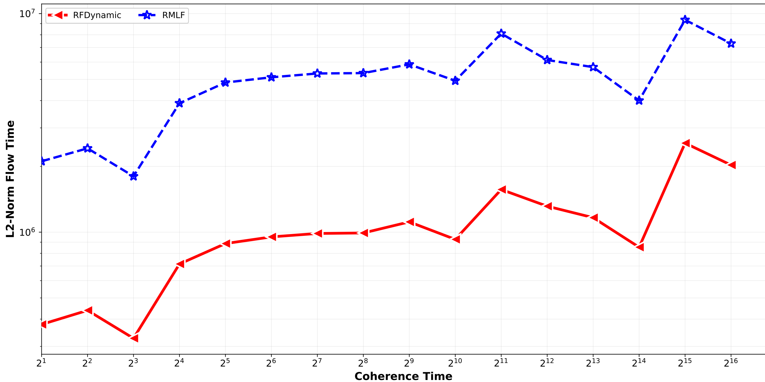
RFDynamic vs RMLF - L2 Norm Flow Time normal_combination_random std6_std9_std12 / triplet_1
