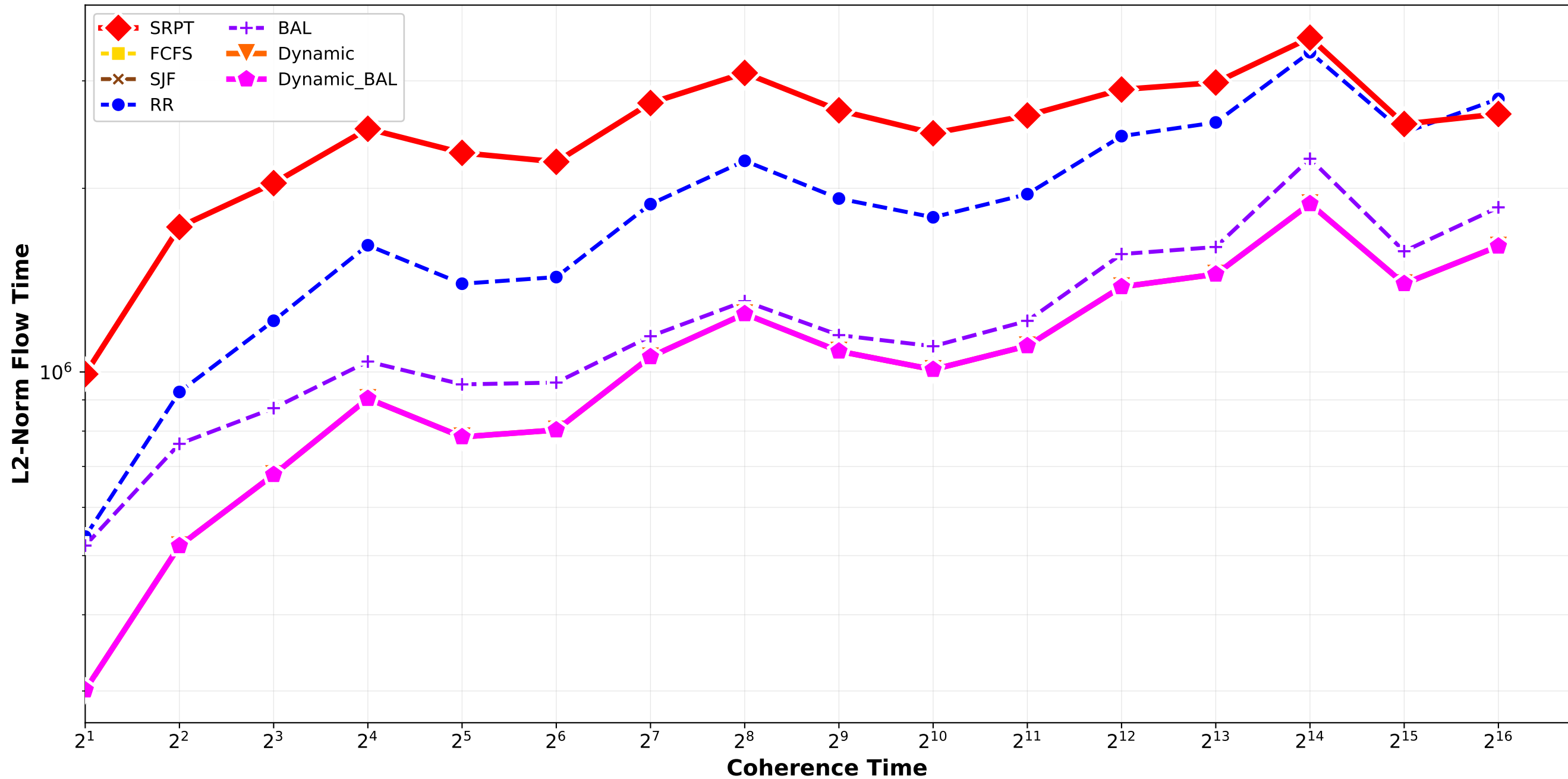
Clairvoyant Algorithms - L2 Norm Flow Time normal_combination_random std9_std12_std15 / triplet_2
