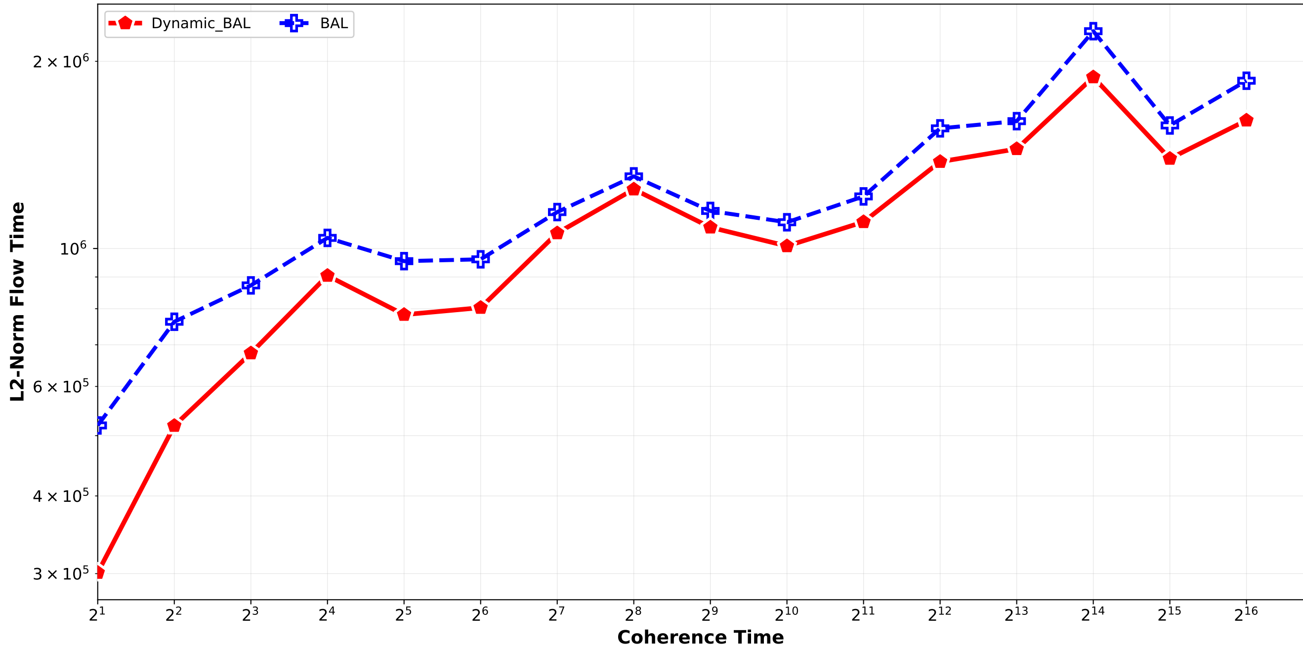
Dynamic_BAL vs BAL - L2 Norm Flow Time normal_combination_random std9_std12_std15 / triplet_2
