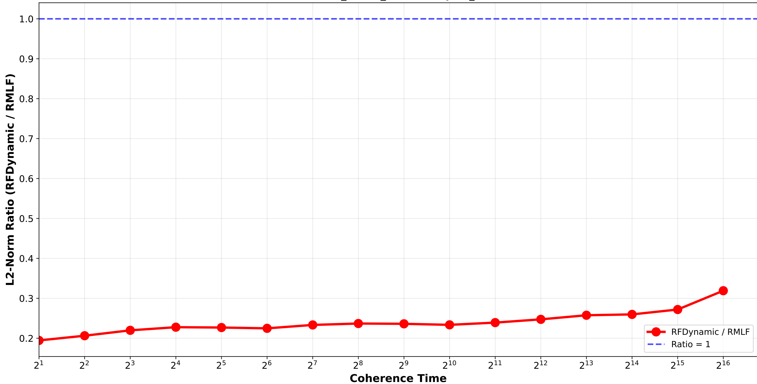
RFDynamic vs RMLF - L2 Norm Ratio normal_combination_random std9_std12_std15 / triplet_2
