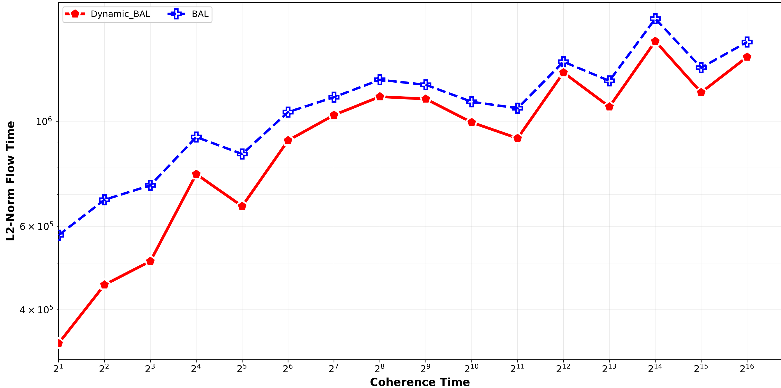
Dynamic_BAL vs BAL - L2 Norm Flow Time normal_combination_random std12_std15 / pair_3
