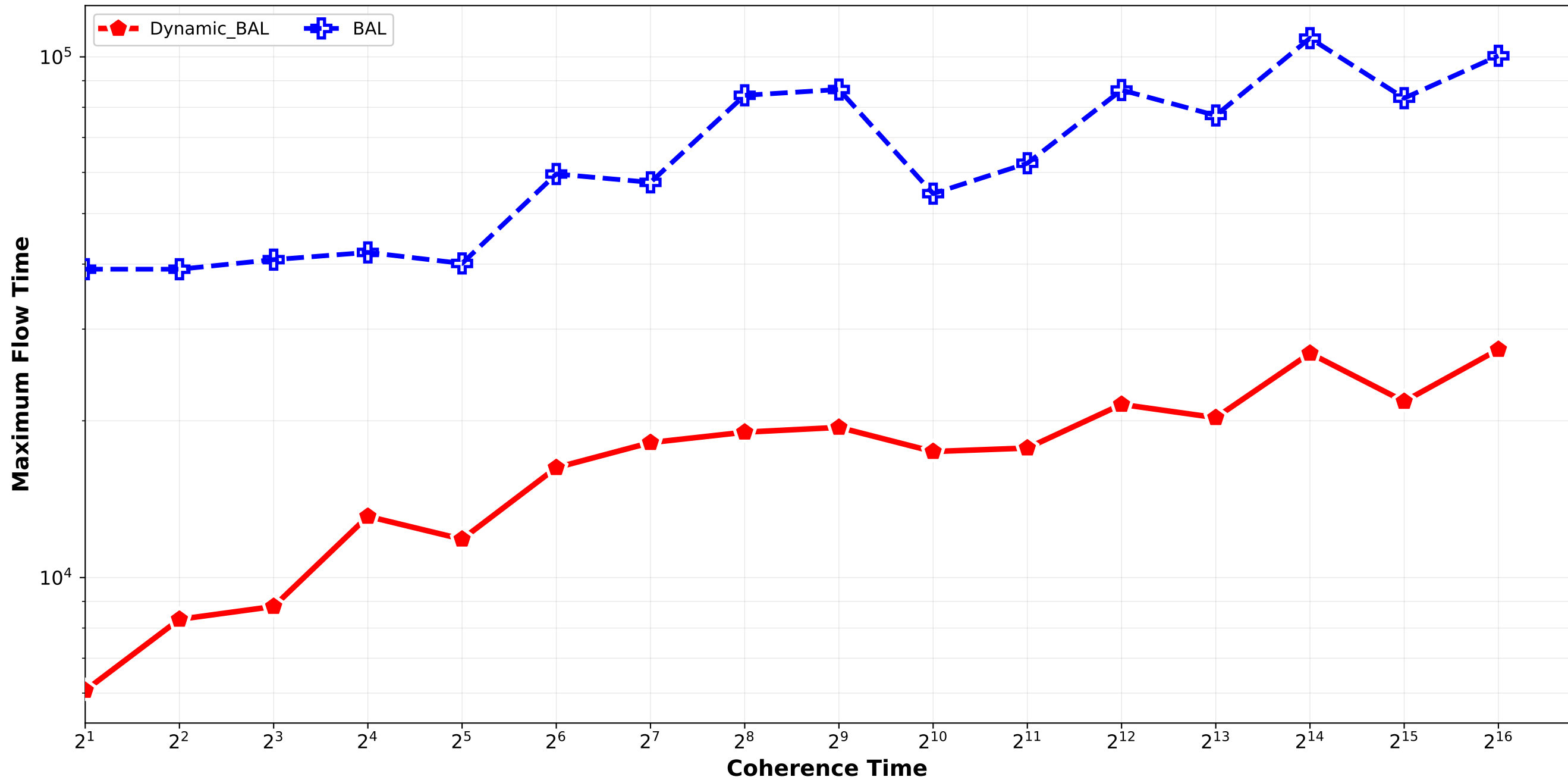
Dynamic_BAL vs BAL - Maximum Flow Time normal_combination_random std12_std15 / pair_3
