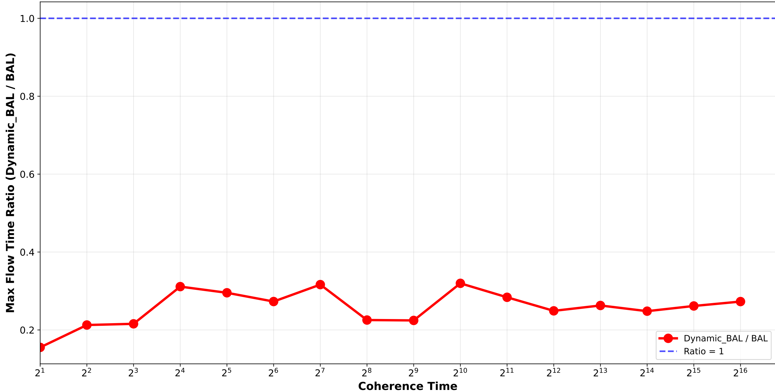
Dynamic_BAL vs BAL - Max Flow Time Ratio normal_combination_random std12_std15 / pair_3
