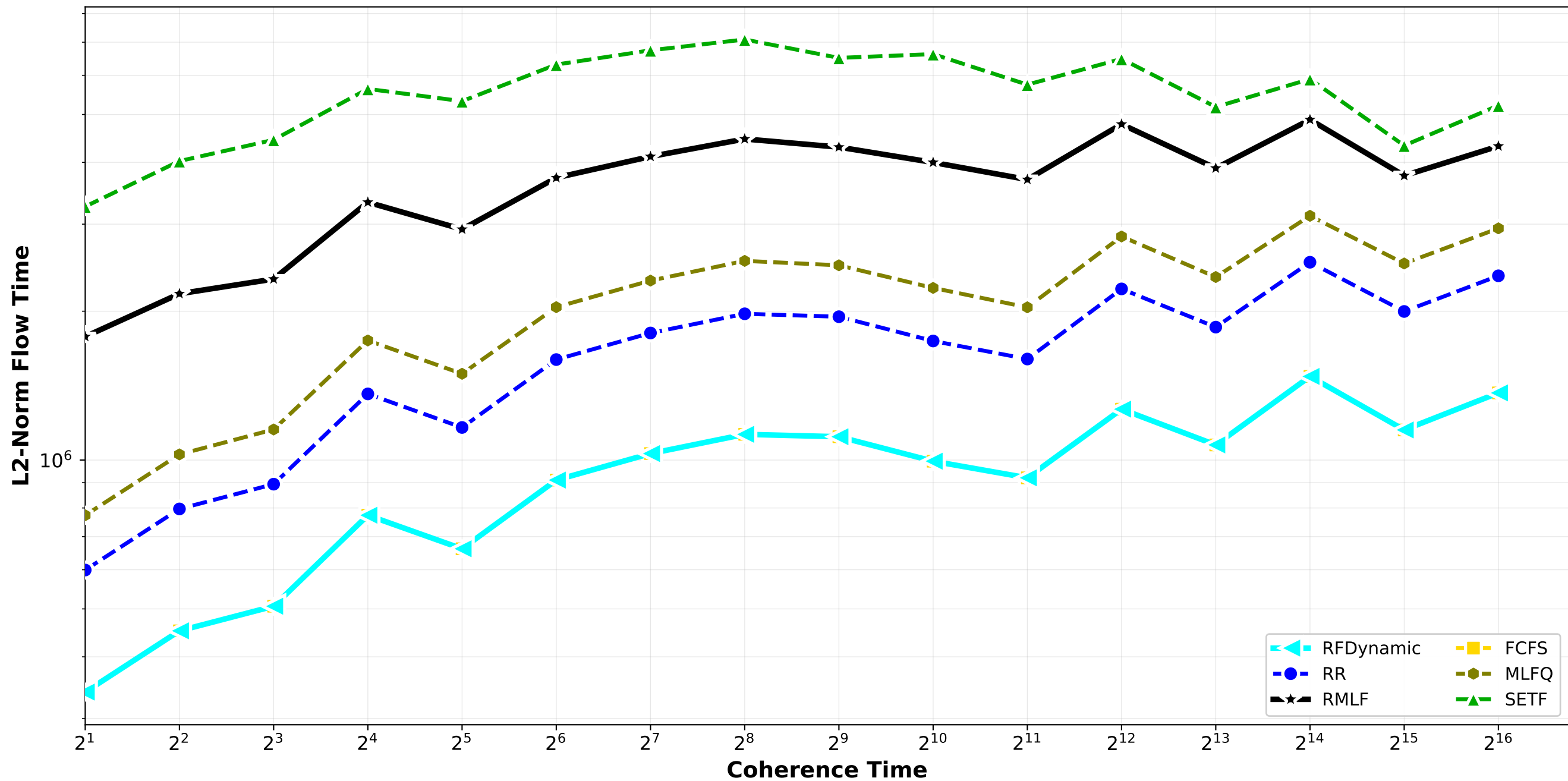
Non-Clairvoyant Algorithms - L2 Norm Flow Time normal_combination_random std12_std15 / pair_3
