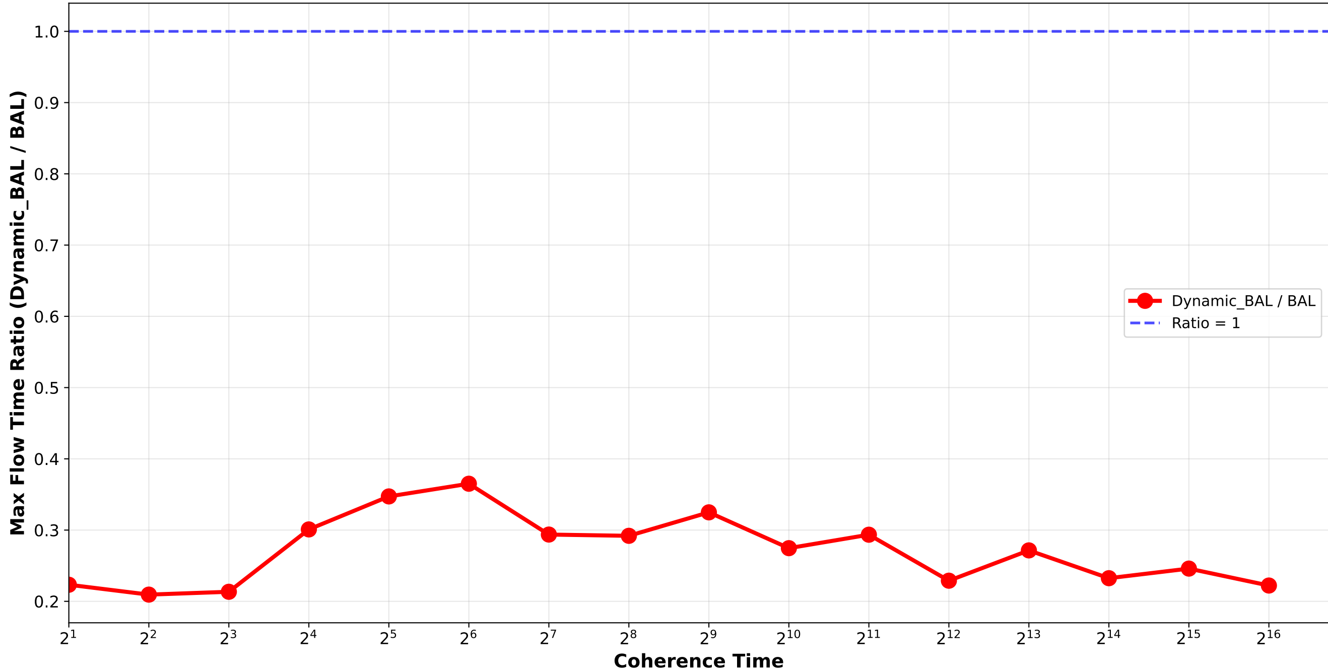
Dynamic_BAL vs BAL - Max Flow Time Ratio normal_combination_random std15_std18 / pair_4
