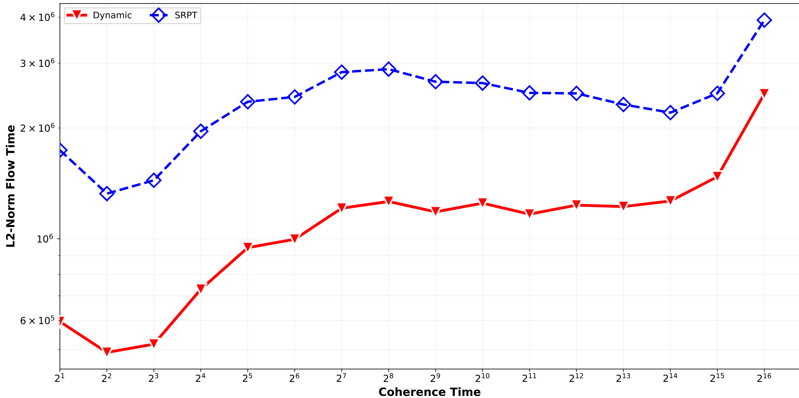
Dynamic vs SRPT - L2 Norm Flow Time normal_combination_random std15_std18 / pair_4
