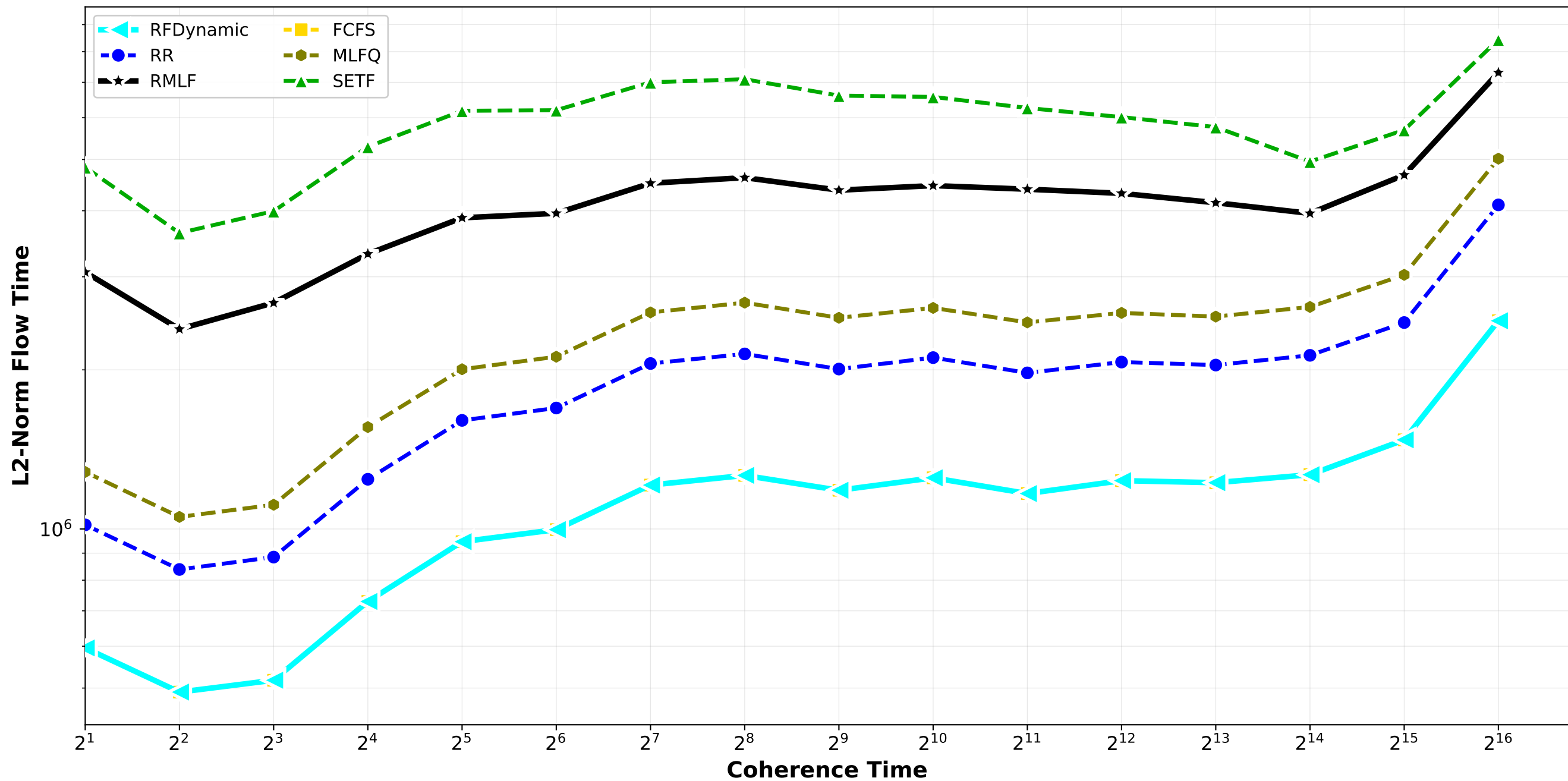
Non-Clairvoyant Algorithms - L2 Norm Flow Time normal_combination_random std15_std18 / pair_4
