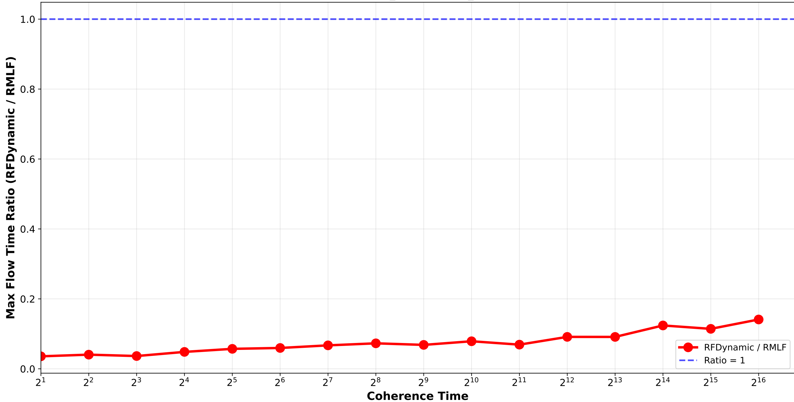
RFDynamic vs RMLF - Max Flow Time Ratio normal_combination_random std15_std18 / pair_4
