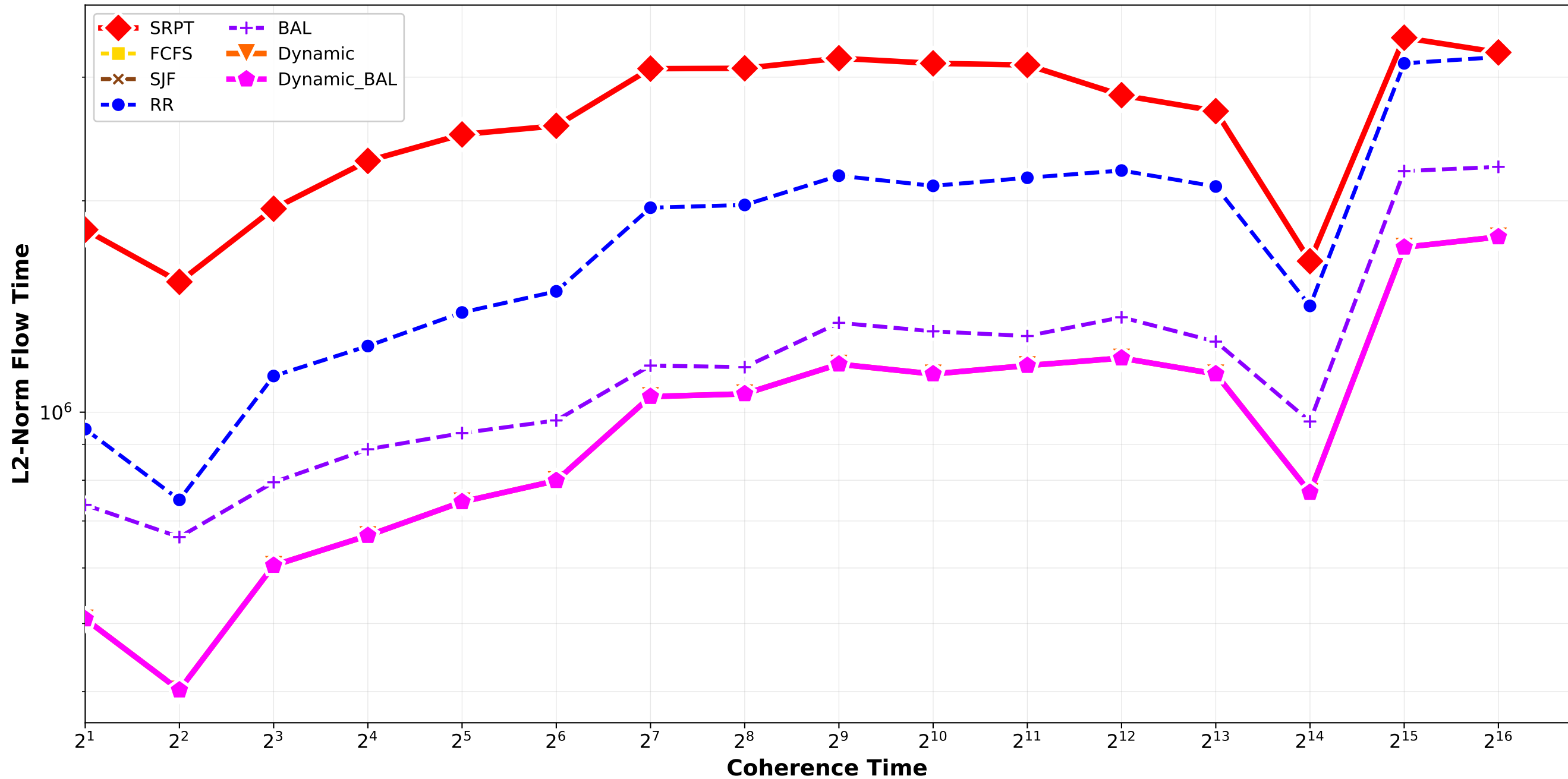
Clairvoyant Algorithms - L2 Norm Flow Time normal_combination_random std6_std9 / pair_1
