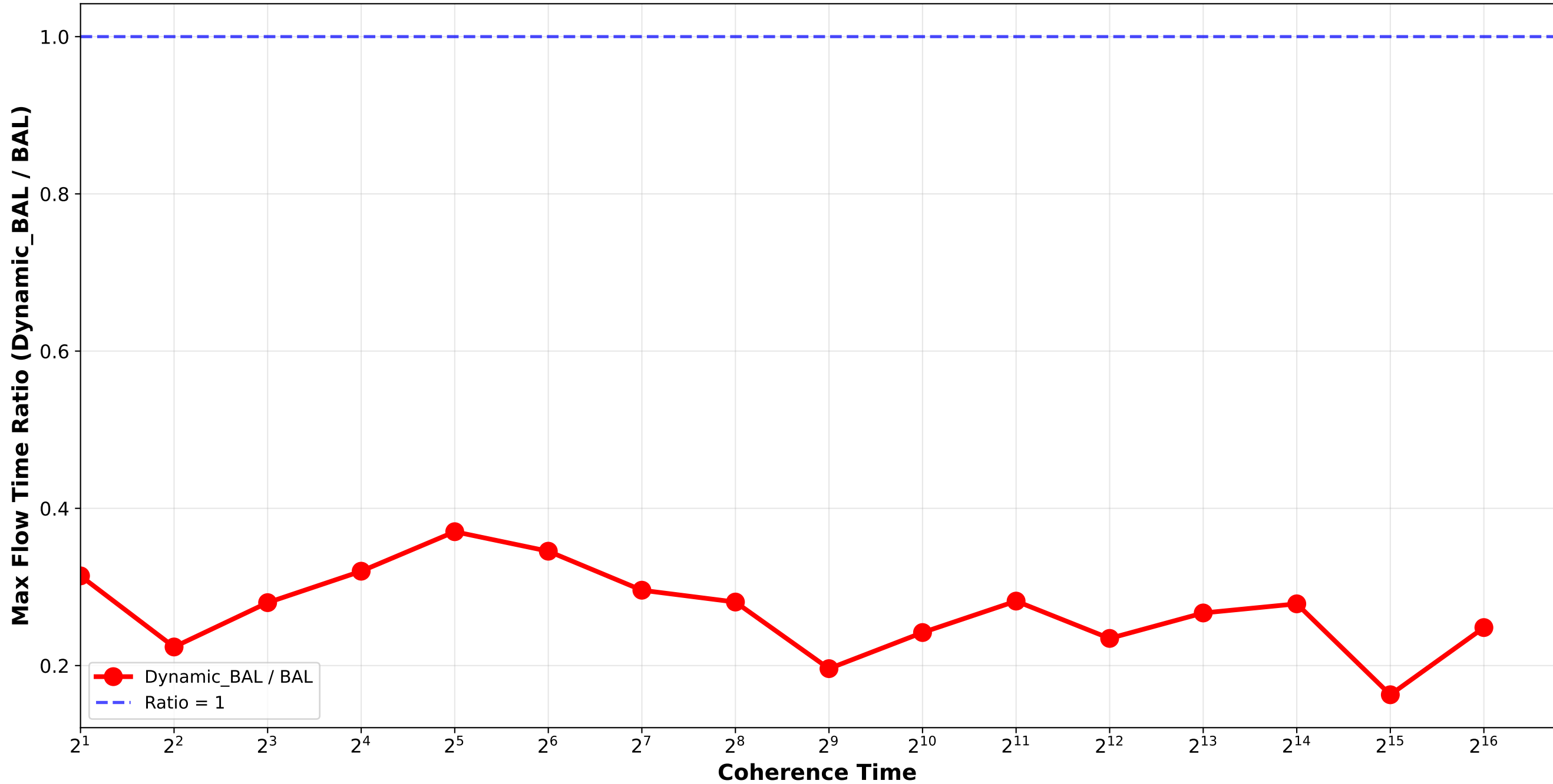
Dynamic_BAL vs BAL - Max Flow Time Ratio normal_combination_random std6_std9 / pair_1
