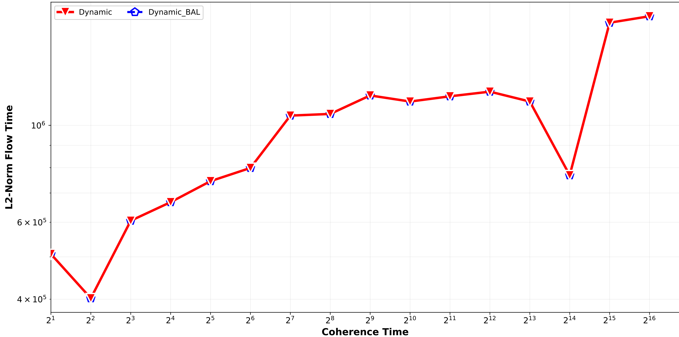
Dynamic vs Dynamic_BAL - L2 Norm Flow Time normal_combination_random std6_std9 / pair_1
