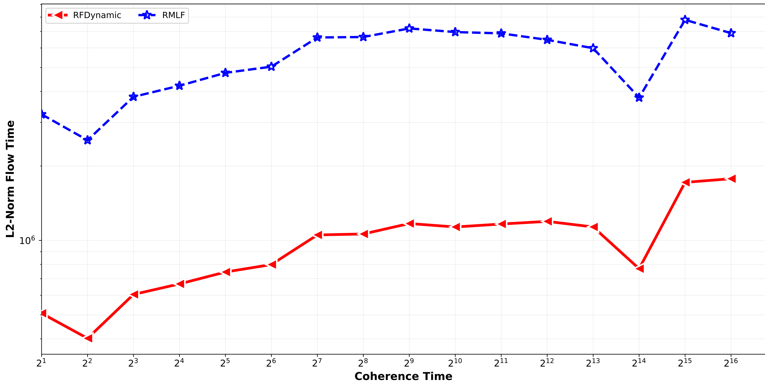
RFDynamic vs RMLF - L2 Norm Flow Time normal_combination_random std6_std9 / pair_1
