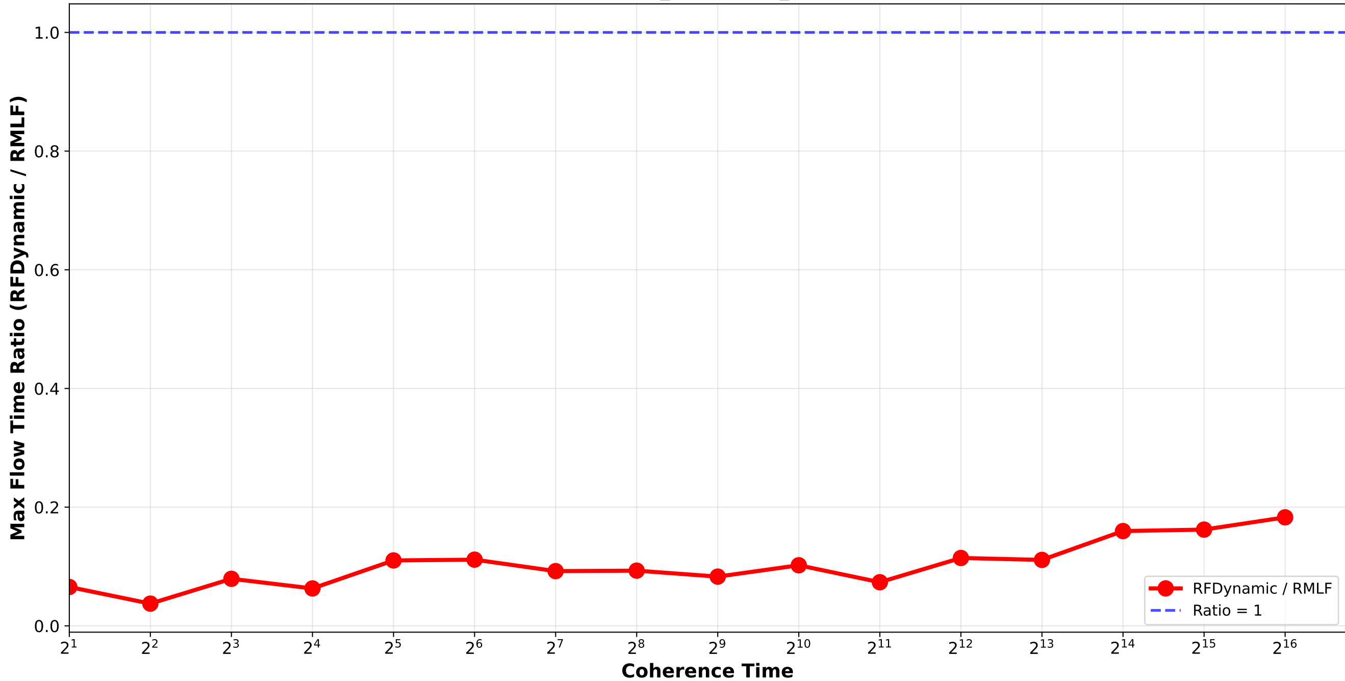
RFDynamic vs RMLF - Max Flow Time Ratio normal_combination_random std6_std9 / pair_1
