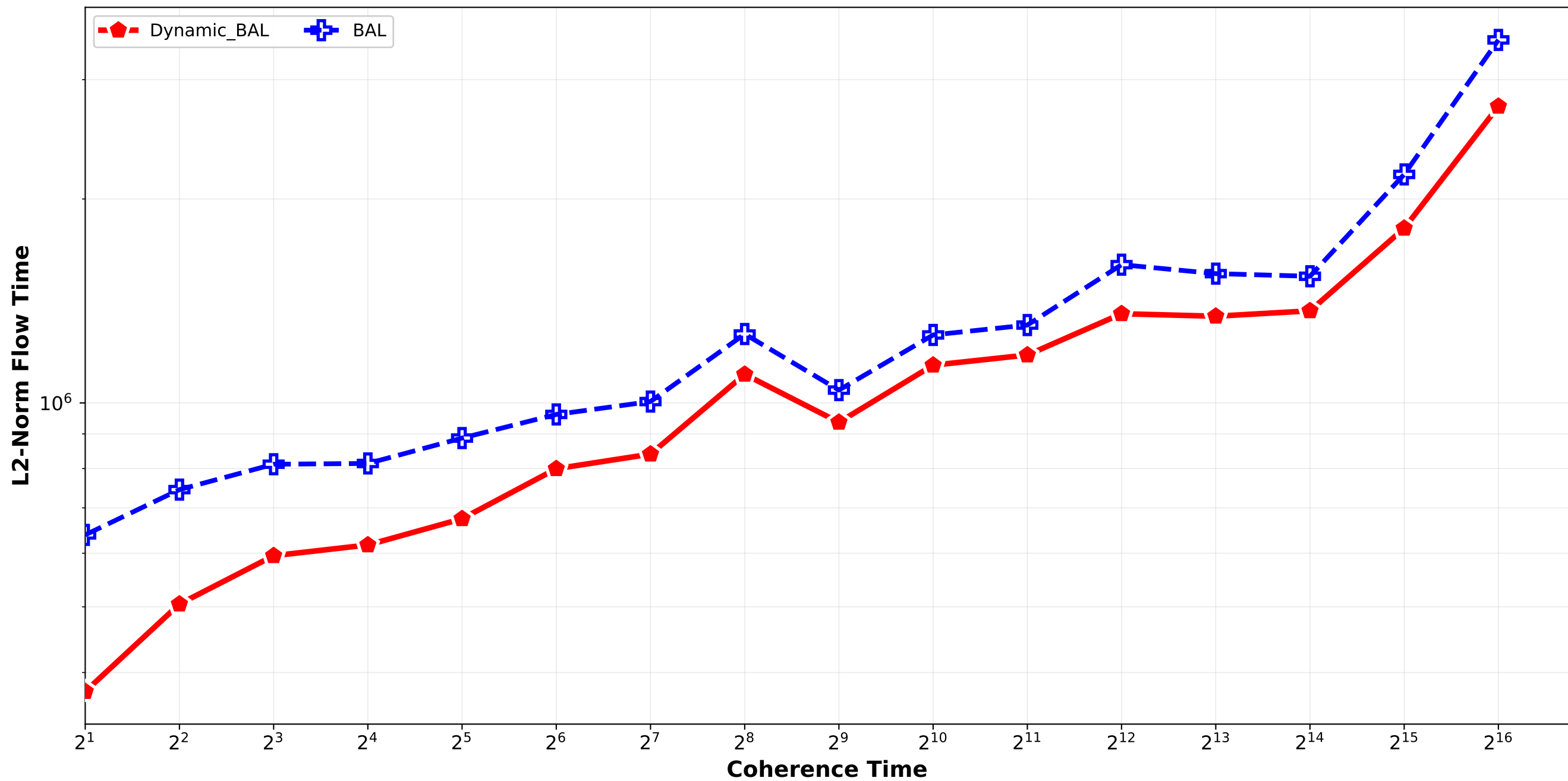
Dynamic_BAL vs BAL - L2 Norm Flow Time normal_combination_random std9_std12 / pair_2
