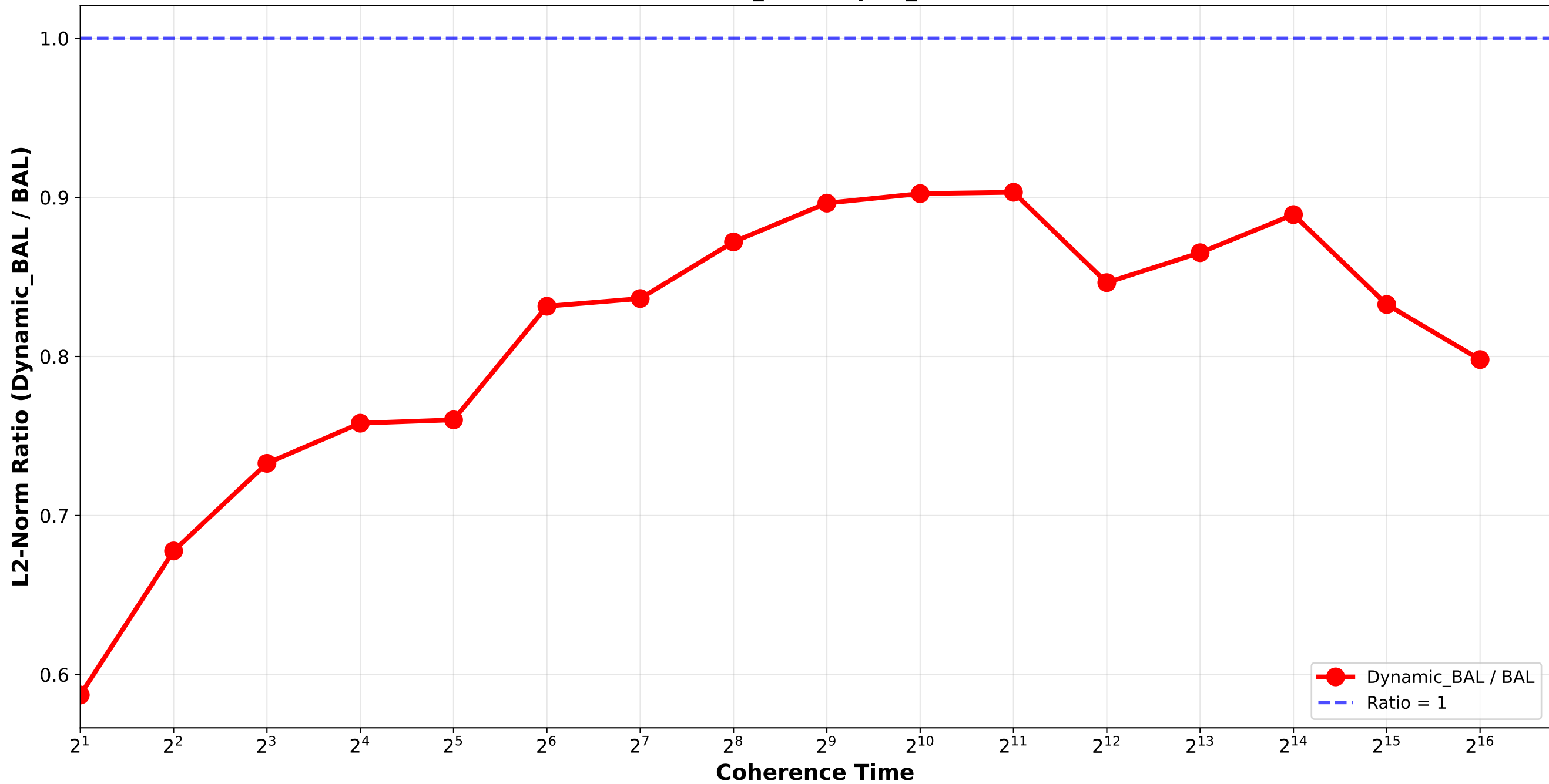
Dynamic_BAL vs BAL - L2 Norm Ratio normal_combination_random std9_std12 / pair_2
