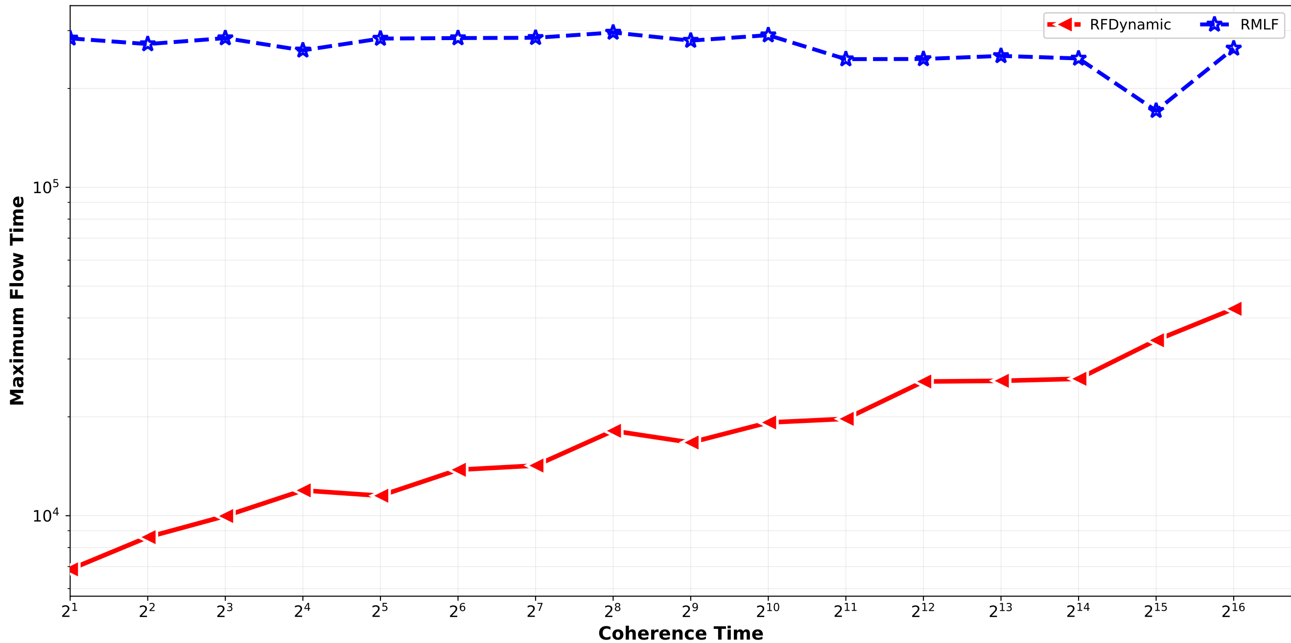
RFDynamic vs RMLF - Maximum Flow Time normal_combination_random std9_std12 / pair_2
